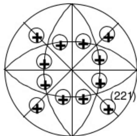
5- Trisoctahedron
