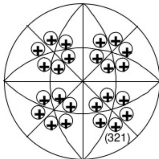
7- Hexaoctahedron
