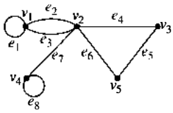
FIGURE 7 A Pseudograph.
