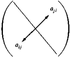
FIGURE 2 A Symmetric Matrix.
