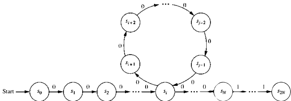
FIGURE 6 The Path Produced by 0^{N+t} 1^N .
