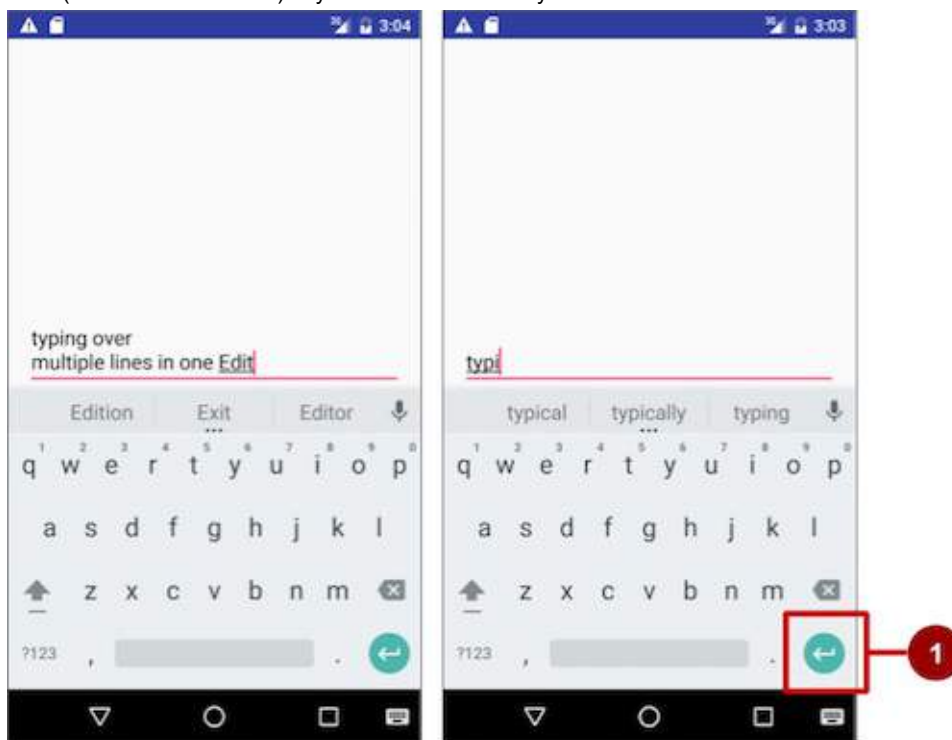
EditText view.
