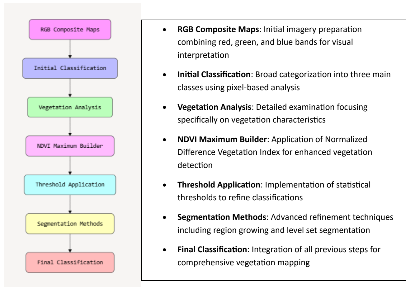
Fig.10. NDVI Process
