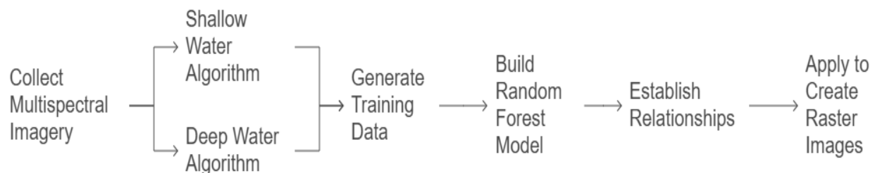
Fig.7. Flowchart for Water Temperature and Turbidity Retrieval Process
