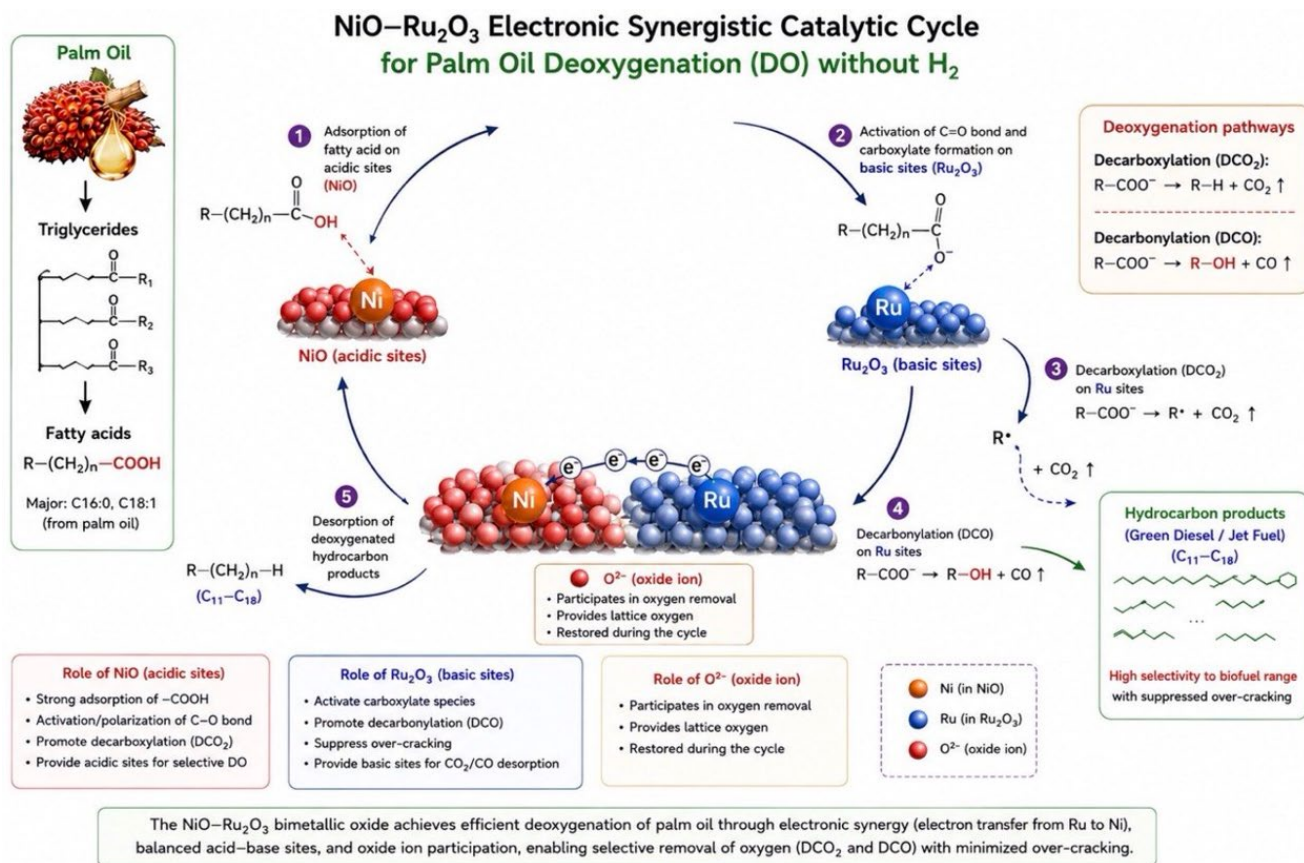
Figure 11. Proposed electronic synergistic catalytic mechanism of the NiO– \text{Ru}_2\text{O}_3 /DS catalyst during palm oil deoxygenation.
