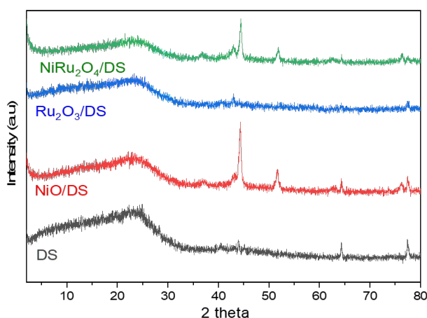
Figure 1. XRD patterns for new catalysts.
