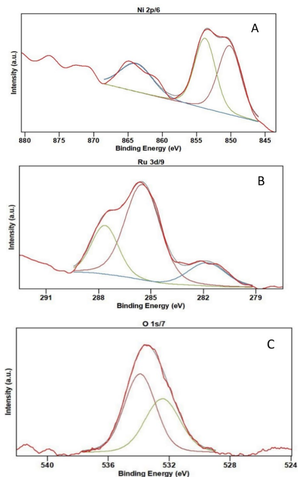
Figure 9. XPS spectra of the synthesized \text{NiRu}_2\text{O}_4 supported on date seeds (DS).
