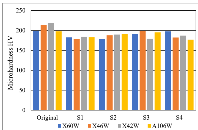
Fig. 8 Microhardness value changes for welded pipes (X42, X46, X60, and ASTM A106) before and after immersion.
