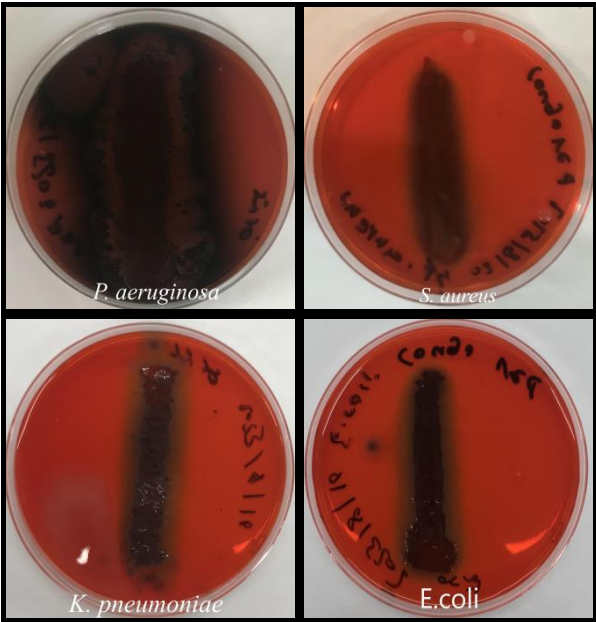
Fig. 6 Detection of biofilms in pathogenic bacteria using Congo red agar
