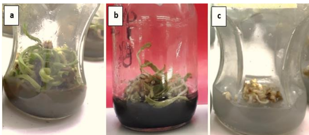
Fig. 3. Bud count after 30 d of cultivation. (a) Medium treated with copper sulfate. (b) Medium treated with zinc oxide. (c) Control treatment.
