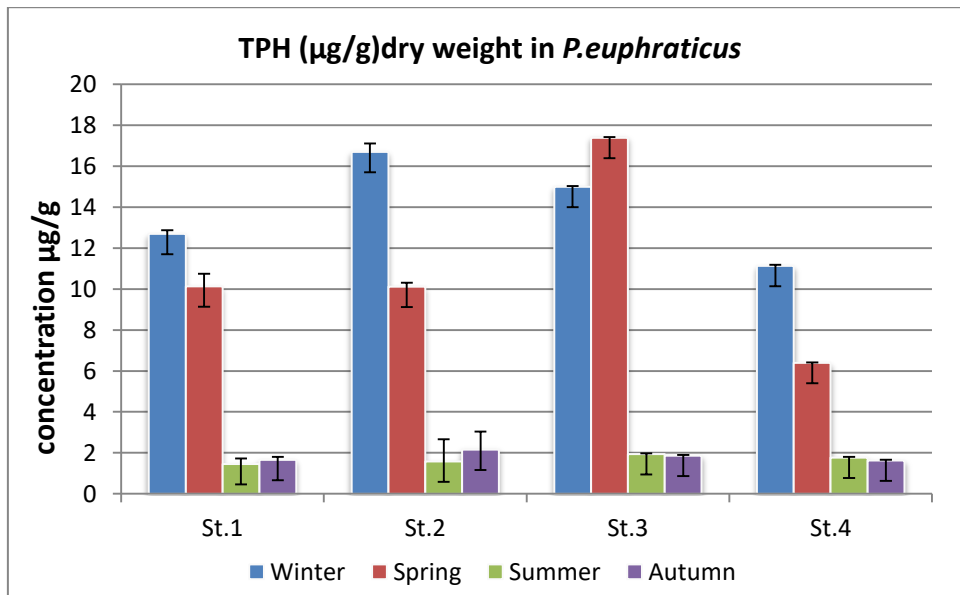
Figur 4: Mean Concentration Of Total Petroleum Hydrocarbons (µg/g) Dry Weight In P.euphraticus
