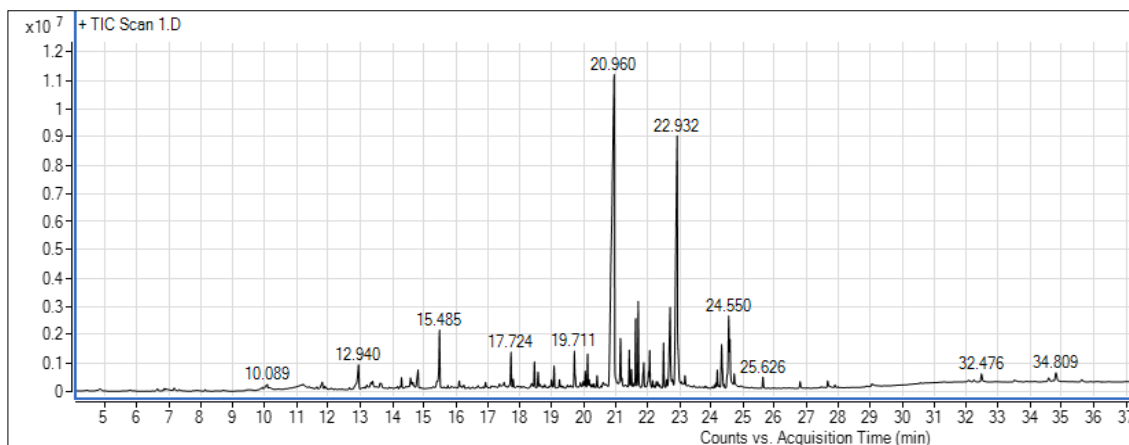
Fig 1: Mass spectrum of the alcoholic extract of E. intestinalis
