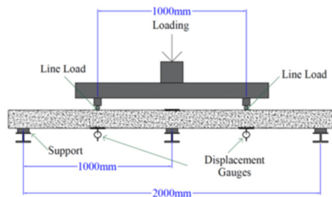
Fig. 3. Testing scheme.
