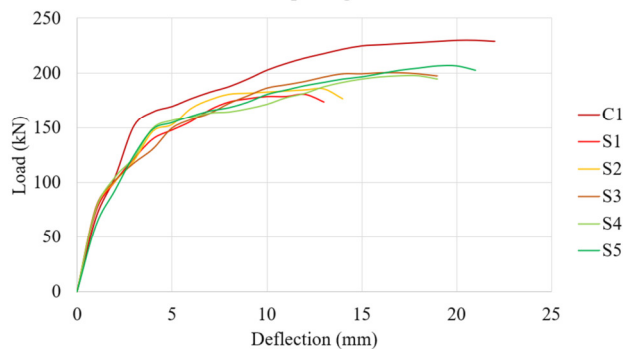
Fig. 6. Load-deflection curves according to opening location.
