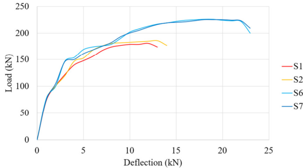
Fig. 10. Load-Deflection curve of additional reinforcement.
