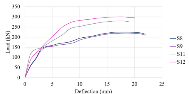
Fig. 9. Load-deflection curves with opening in one of two spans.
