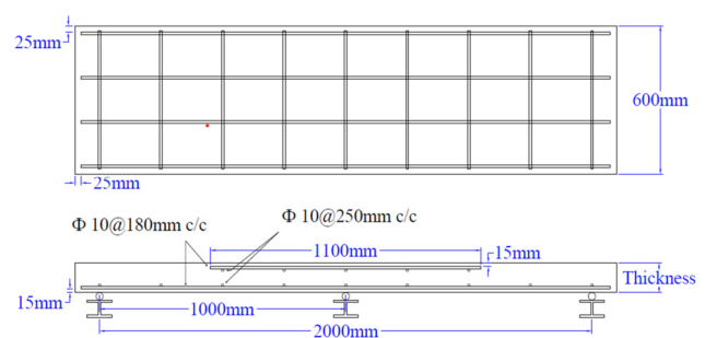
Fig. 1. Reinforcement details of slab.
