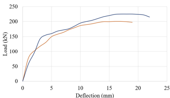
Fig. 7. Load-deflection curves according to opening shape.
