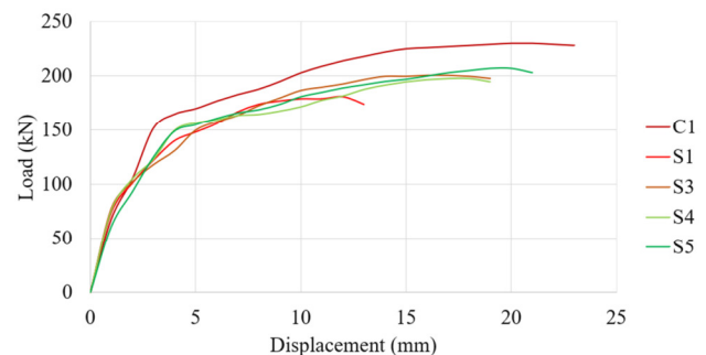
Fig. 5. Load-deflection curves according to opening size.
