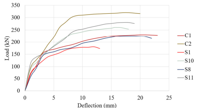
Fig. 8. Load-deflection curves according to opening thickness.
