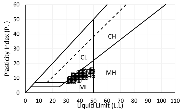
Fig. 7. Plasticity chart for Ammarah soil.
