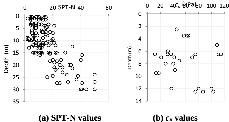
Fig. 5. Variation of soil strength with depth.
