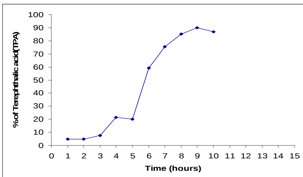
Figure 2: Effect of time on percentage yield of TPA at 132°C
