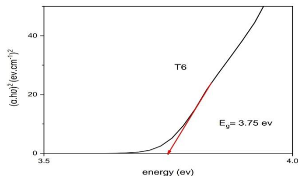
Fig. 10: Energy band gap for compound T6 by Tauc plot.
