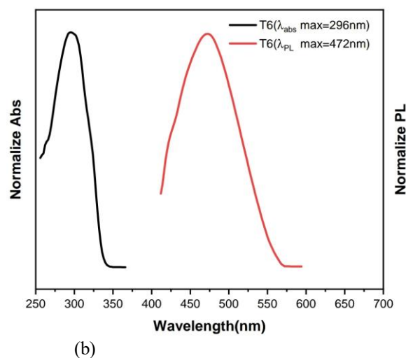
Fig. 4: Absorbance and emission spectrum of compounds C3 and T6.
