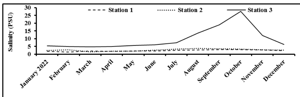
Figure 3. Monthly variations in the salinity in the three stations of the Shatt Al-Arab River.
