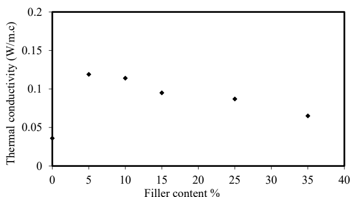
Fig. 11. The relationship between thermal conductivity and weight ratios coal powder added to polyurethane polymer
