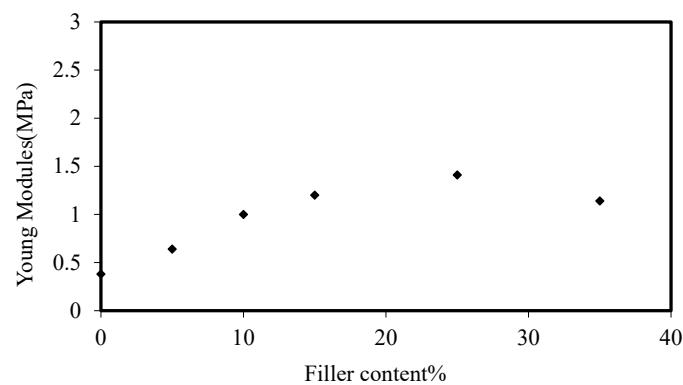
Fig. 8. The relationship between Young modules and weight ratios coal powder additive to polymer
