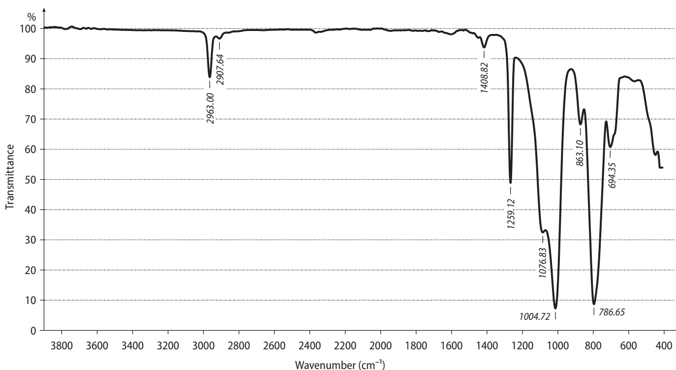
Fig. 1. FTIR of the soft liner before the addition of nano-CuO
