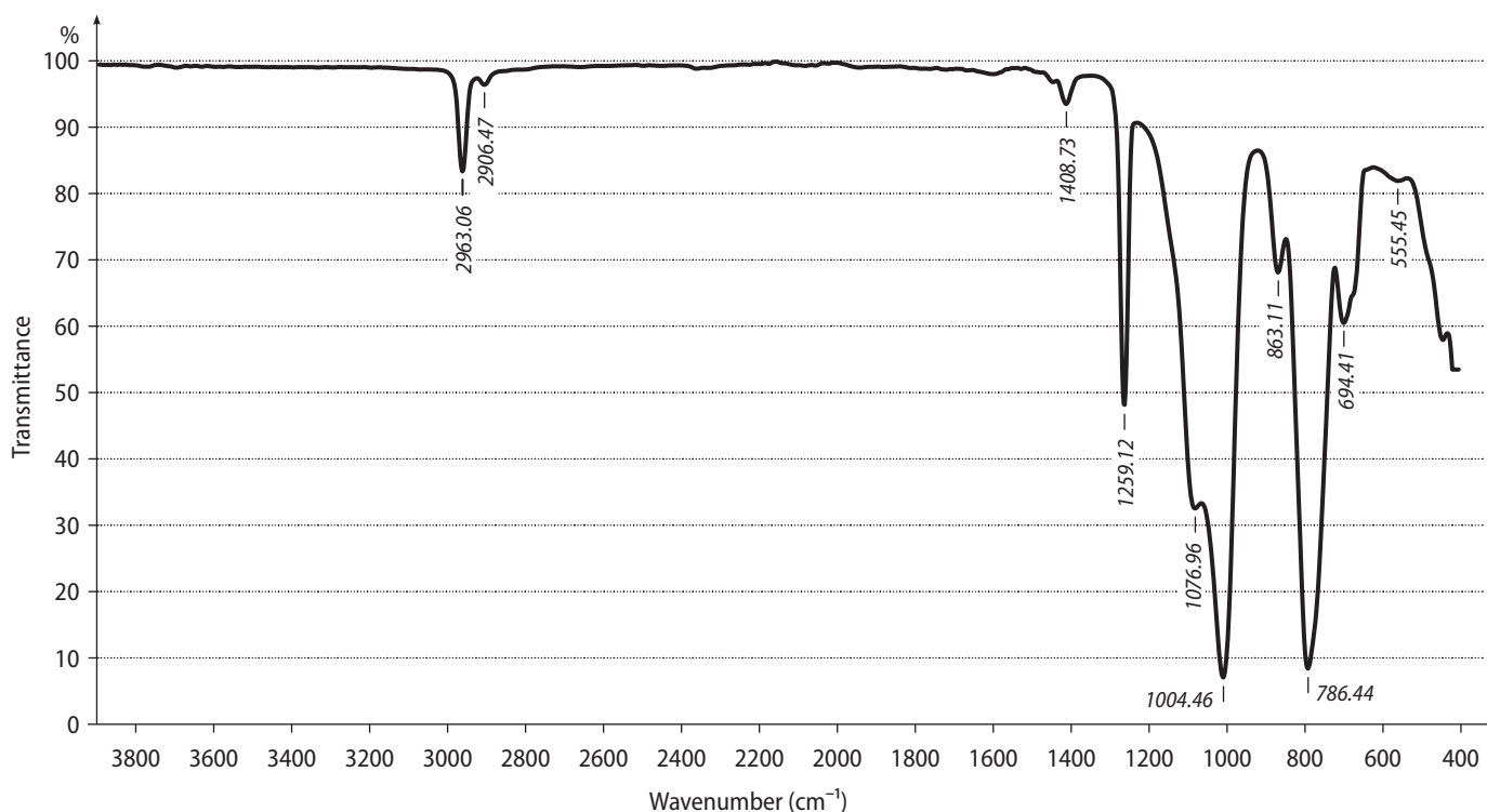
Fig. 2. FTIR of the soft liner after adding nano-CuO
