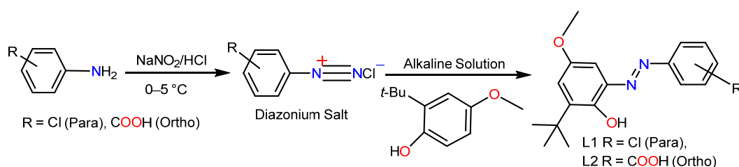
Fig 1. Synthesis of azo compounds L1 and L2
