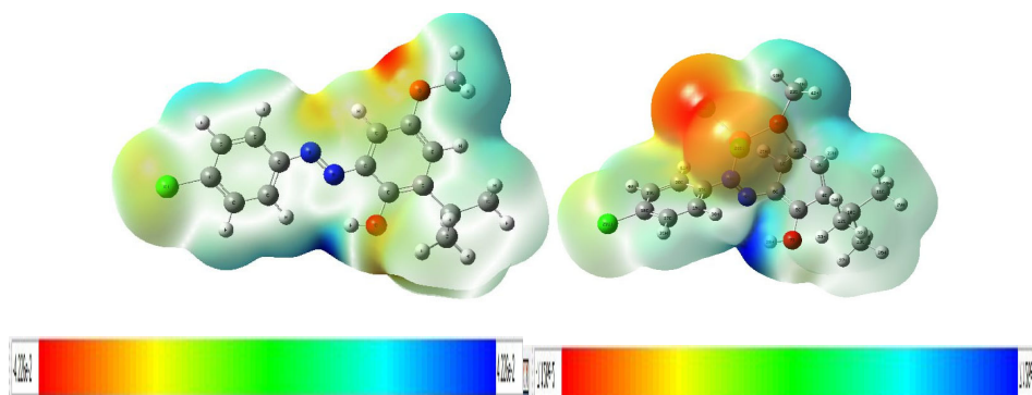
Fig 3. Electronic surface potential of (a) L1 ((-4.22) – (+4.22) au) and (b) [CuCl 2 (L1)] ((-7.12) – (+7.12) au)
