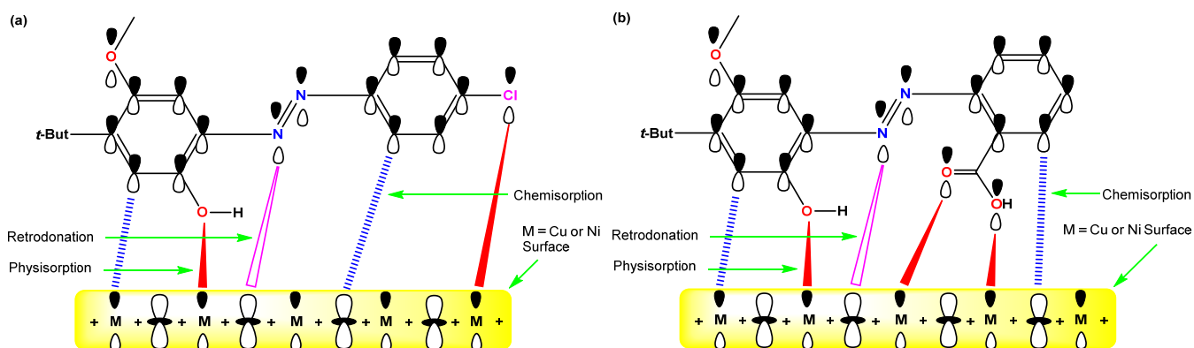
Fig 6. Proposed corrosion inhibition mechanism of inhibitor (a) L1 and (b) L2 with metal surface
