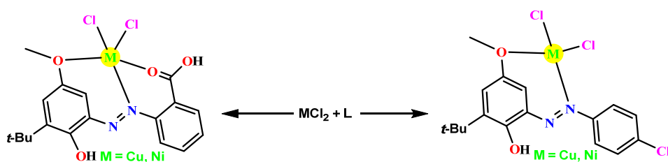
Fig 2. Synthesis of azo metal complexes
