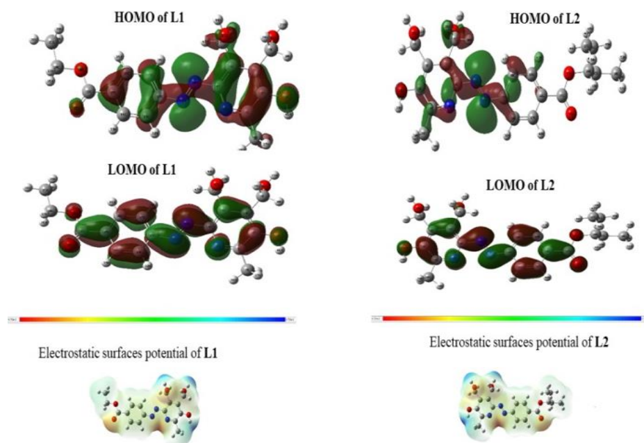
Figure 9. HOMO, LOMO, and Electrostatic surfaces potential of L1 and L2
