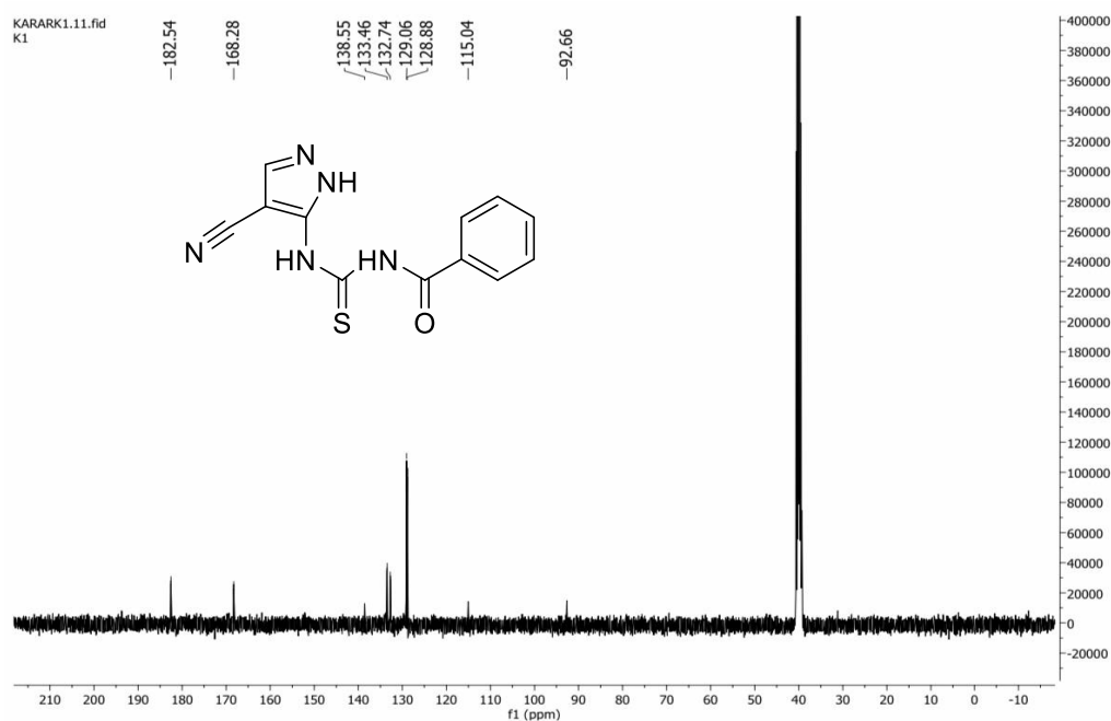
Figure 6. The 13 C- NMR spectrum of VIa
