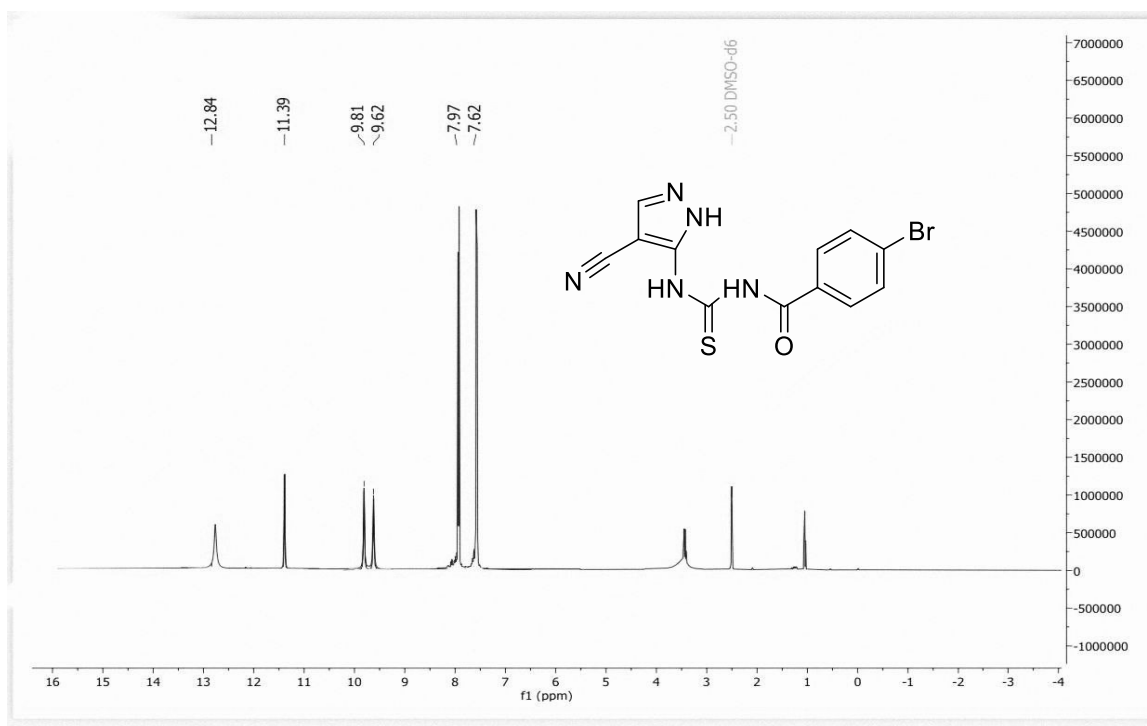
Figure 13. The 1 H - NMR spectrum of VIc
