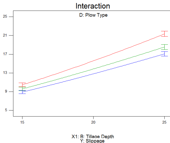
Fig. (13): Effect of tillage depth, plow type and their interaction on the slippage percentage.
