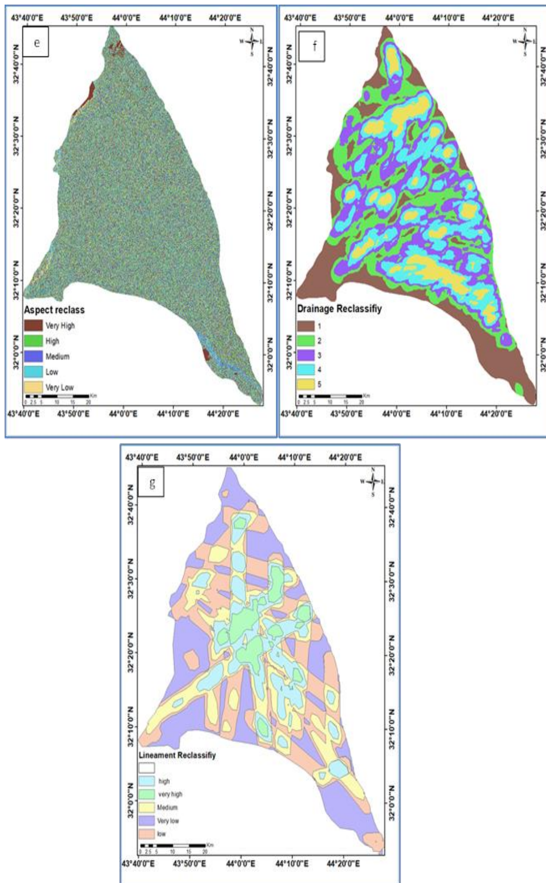
Figure 9: (a, b, c, d, e, f, and g): Reclassify (Geomorphology, Lithology, Slope, Land use, Aspect, Drainage density, and Lineaments density).
