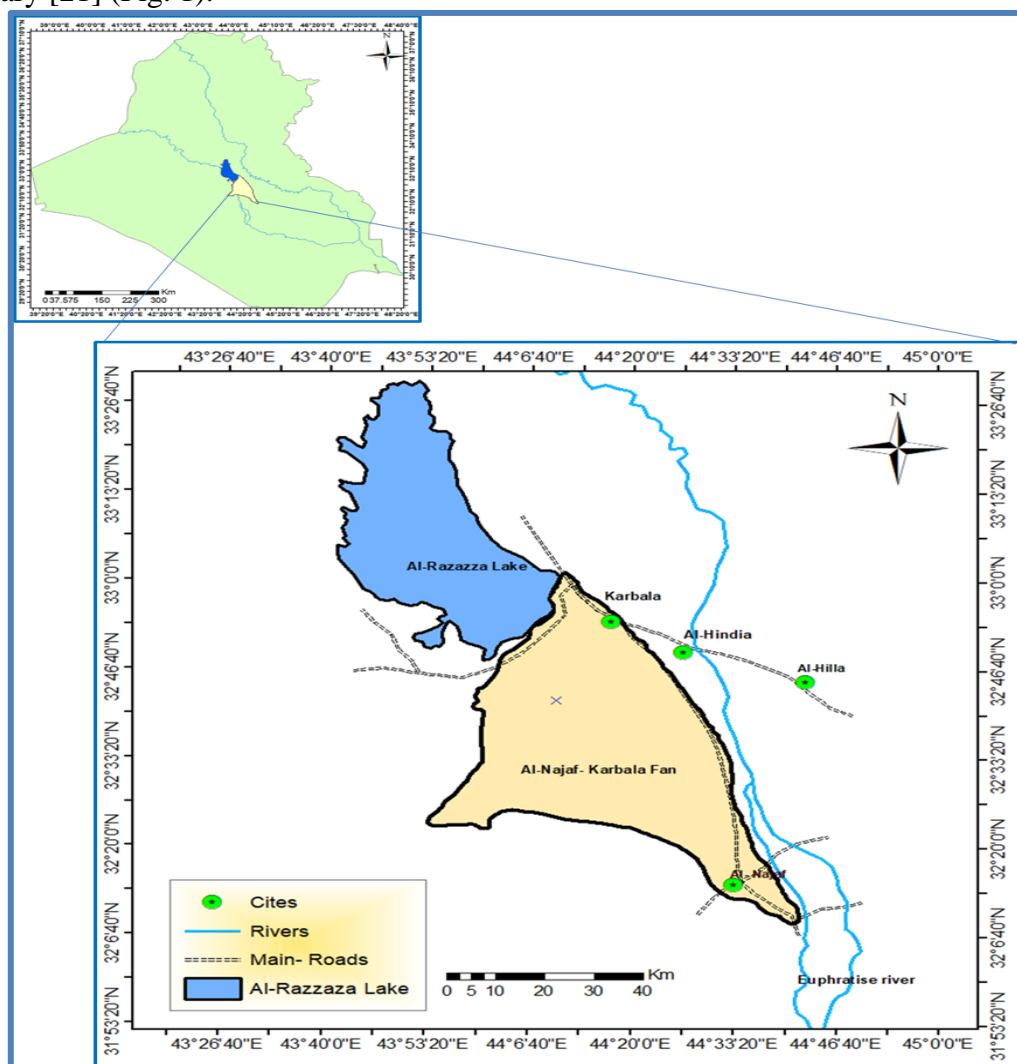
Figure 1: location of study area [22].
