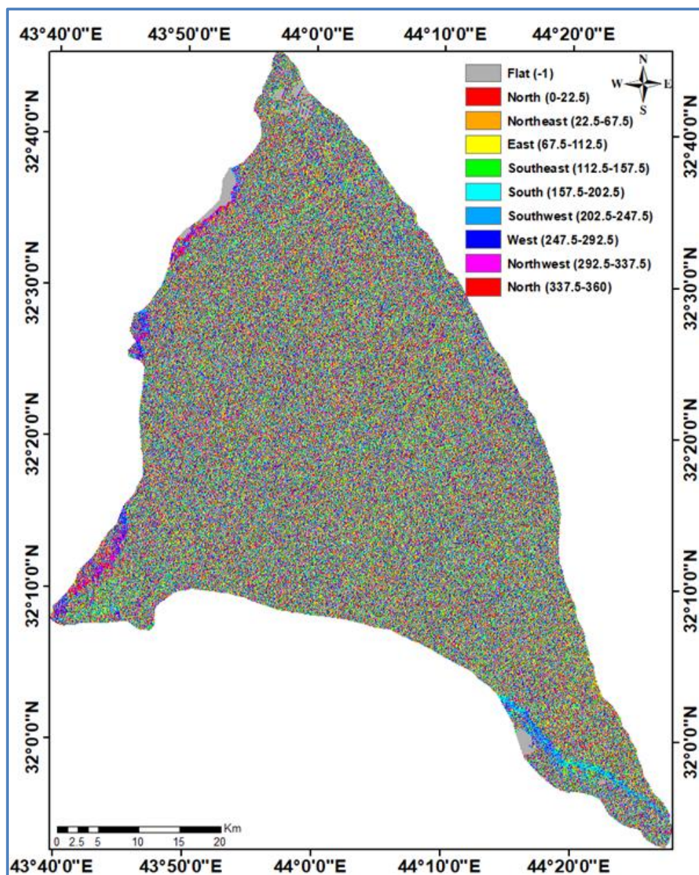
Figure 5 : Aspect map of Al Najaf – Karbala alluvial fan
