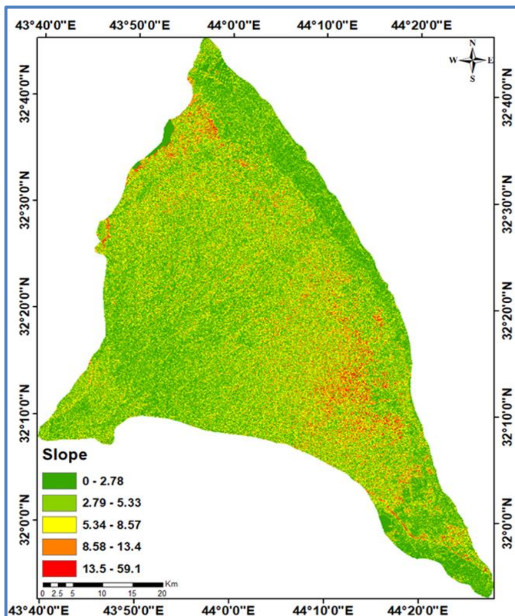
Figure 4: Slope map of Al Najaf – Karbala alluvial fan
