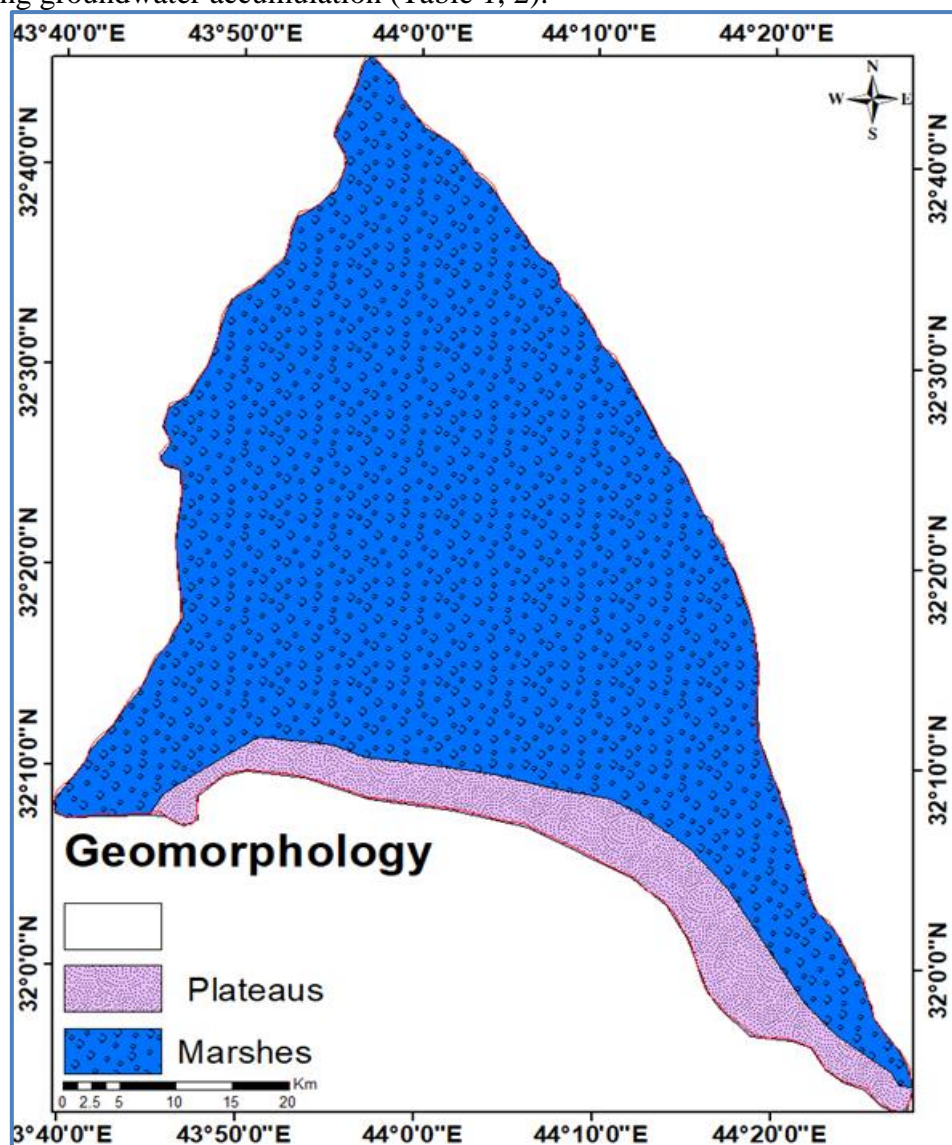
Figure 2: Part from geomorphological map of Al Najaf – Karbala alluvial fan
