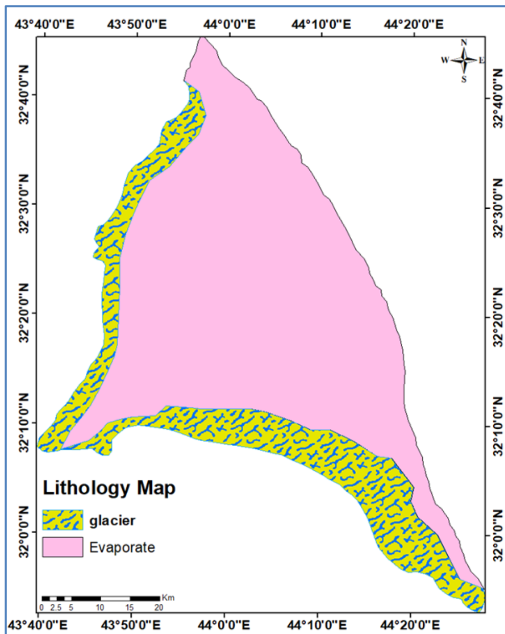
Figure 3: Lithological of Al Najaf – Karbala alluvial fan
