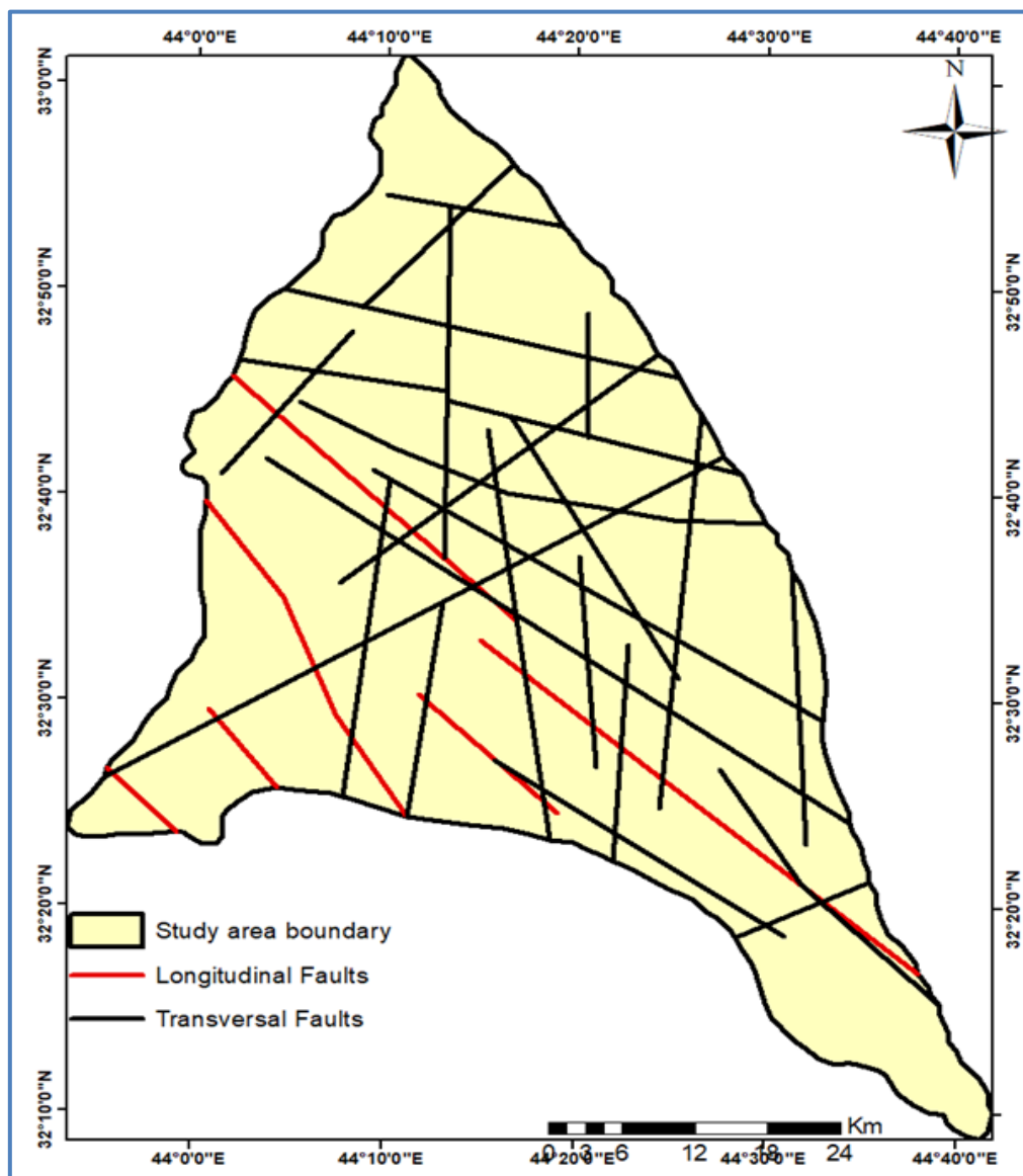
Figure 8: Lineaments map of Al Najaf –Karbala alluvial fan
