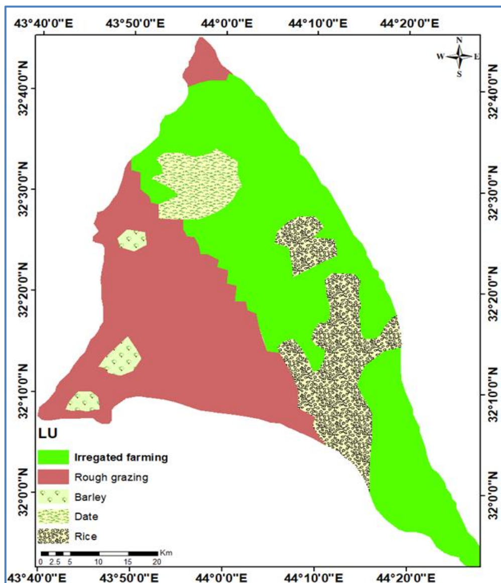
Figure 6: Land Use map of Al Najaf – Karbala alluvial fan
