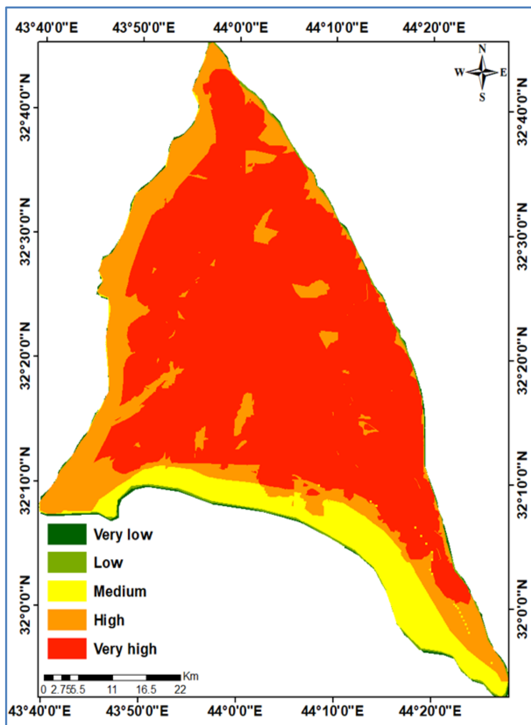
Figure 10: Groundwater potential zone (GWP)
