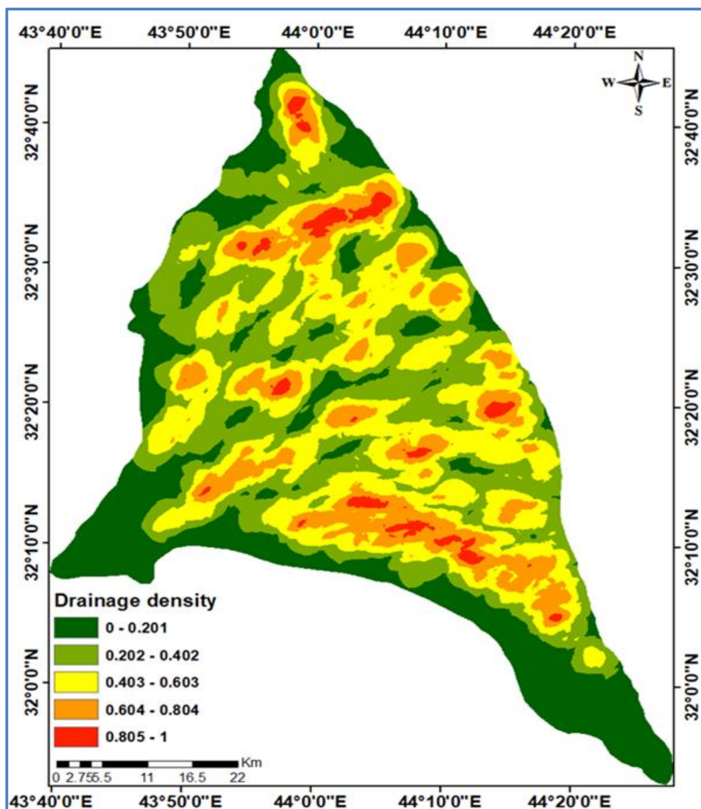
Figure 7: Drainage density map of Al Najaf – Karbala alluvial fan
