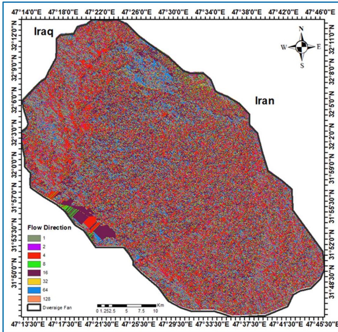
Figure 7: Flow direction map of Dwerige Alluvial fan
