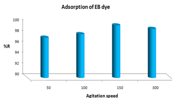
Figure 10. (a) The agitation speed effect on adsorption processes of EB dye
