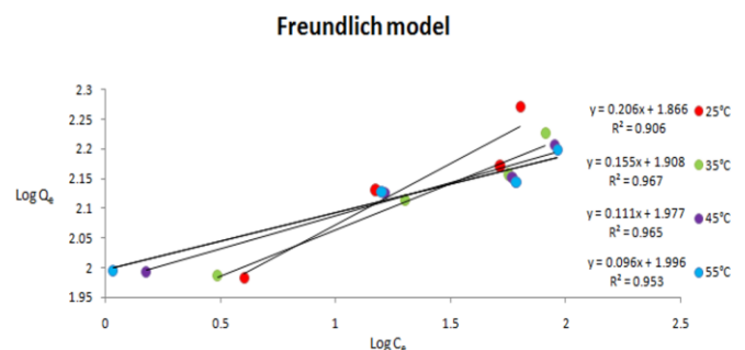
Figure 13. (b) The Freundlich models for EB dye
