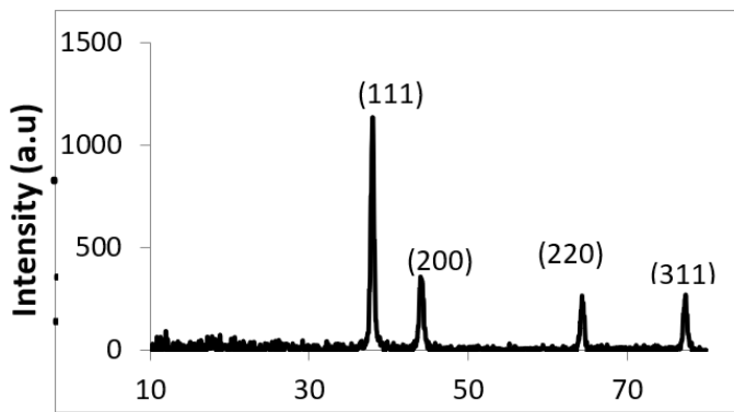
Figure 3. (b) The XRD patterns of the prepared nanocompounds Ag 2 O
