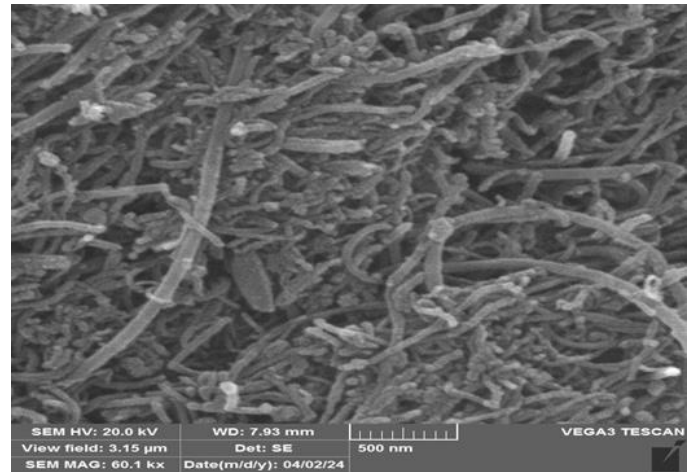
Figure 4. (a) The SEM morphology of nanoparticles sizes
