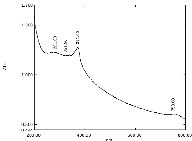
Figure 6. (c) UV Spectra of the prepared nanocompounds ZnO
