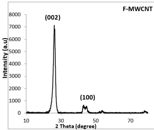
Figure 3. (a) The XRD patterns of the prepared nanocompounds F-MWCNT
