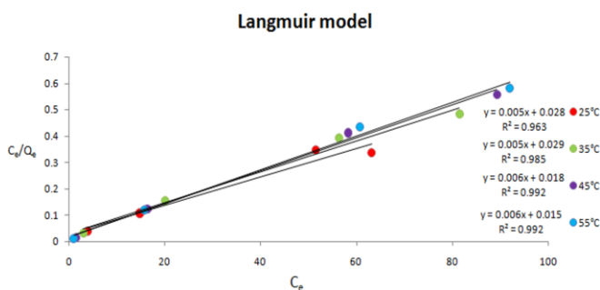
Figure 13. (a) The Langmuir for EB dye
