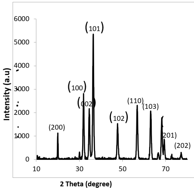
Figure 3. (c) The XRD patterns of the prepared nanocompounds ZnO
