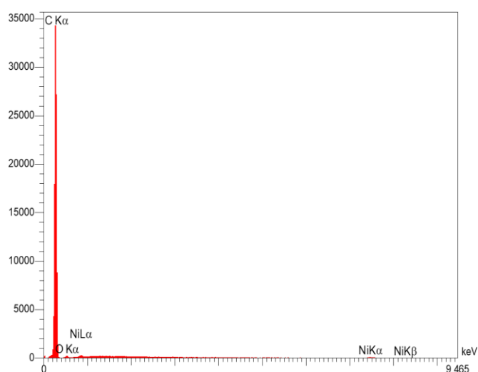
Figure 5. (a) The EDX result of nanocompounds F-MWCNT
