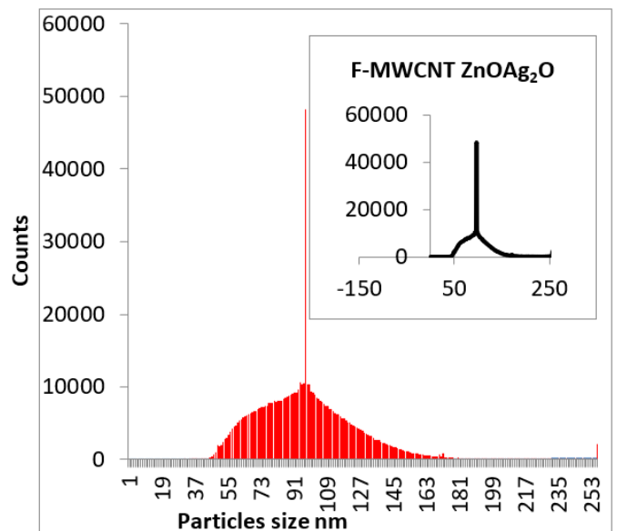
Figure 4. (b) The SEM particles' sizes analyses
