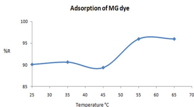
Figure 9. (b) The temperature effect on adsorption processes of MG dye
