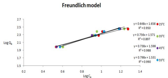
Figure 12. (b) The Freundlich models for MG dye
