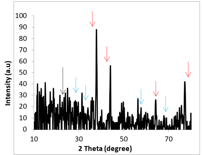
Figure 3. (d) The XRD patterns of the prepared nanocompounds F-MWCNT/ZnOAg 2 O
