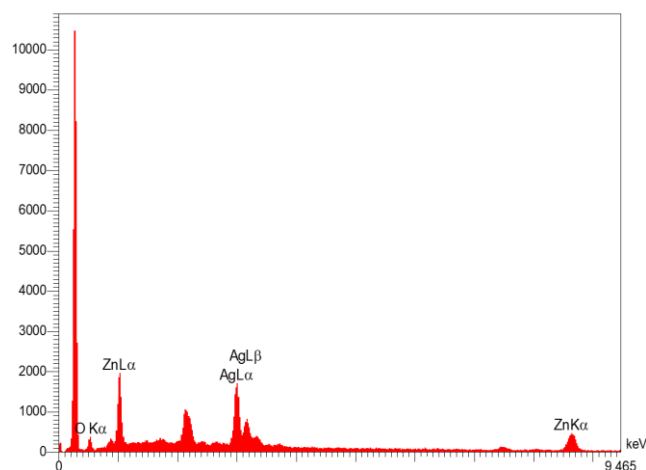
Figure 5. (b) The EDX result of nanocompounds F-MWCNT/ZnOAg 2 O
