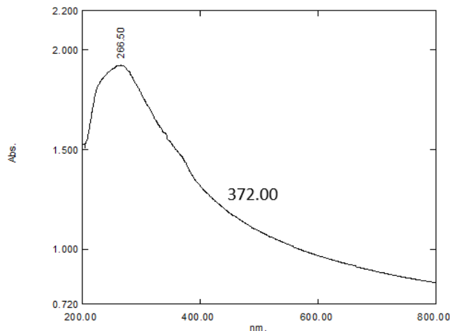
Figure 6. (d) UV Spectra of the prepared nanocompounds F-MWCNTZnOAg 2 O
