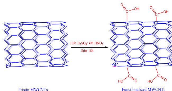
Figure 1. Showed the functionalization of MWCNTs
