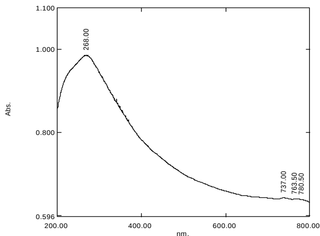
Figure 6. (a) UV Spectra of the prepared nanocompounds F-MWCNT
