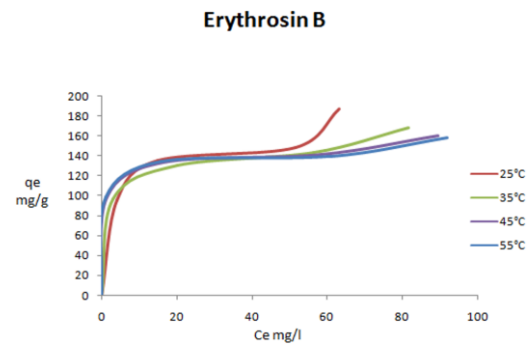
Figure 11. (a) Adsorption isotherm according to Giles classification of EB dye
