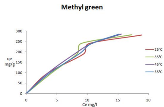
Figure 11. (b) Adsorption isotherm according to Giles classification of MG dye
