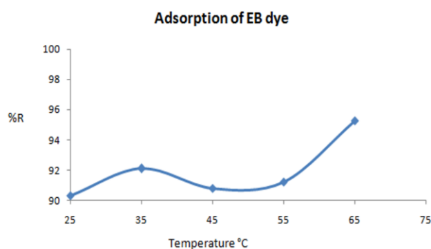
Figure 9. (a) The temperature effect on adsorption processes of EB dye
