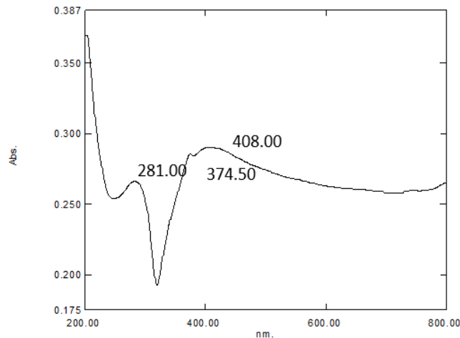
Figure 6. (b) UV Spectra of the prepared nanocompounds Ag 2 O
