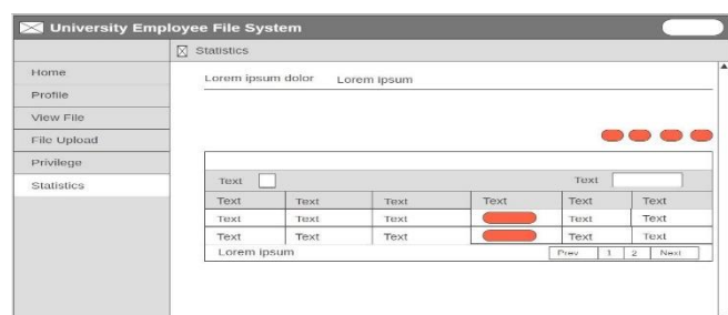
Figure 11: Statistics page
