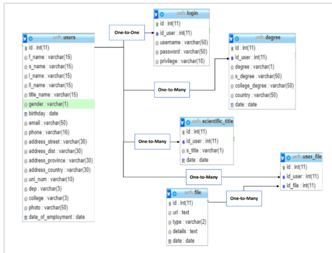
Figure 3: Database schema
