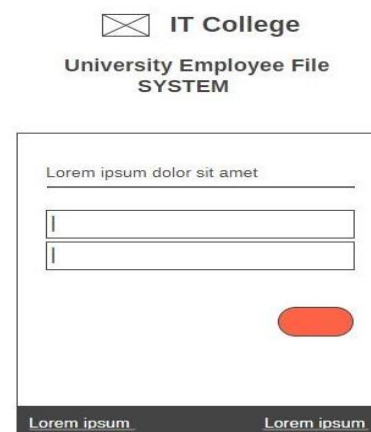
Figure 4: Login page
