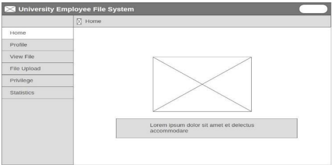
Figure 6: Home page
