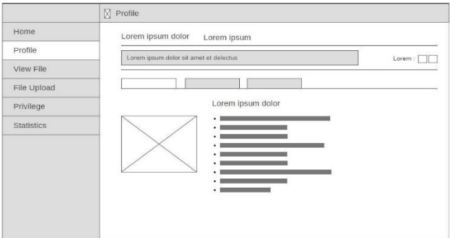
Figure 7: Profile page
