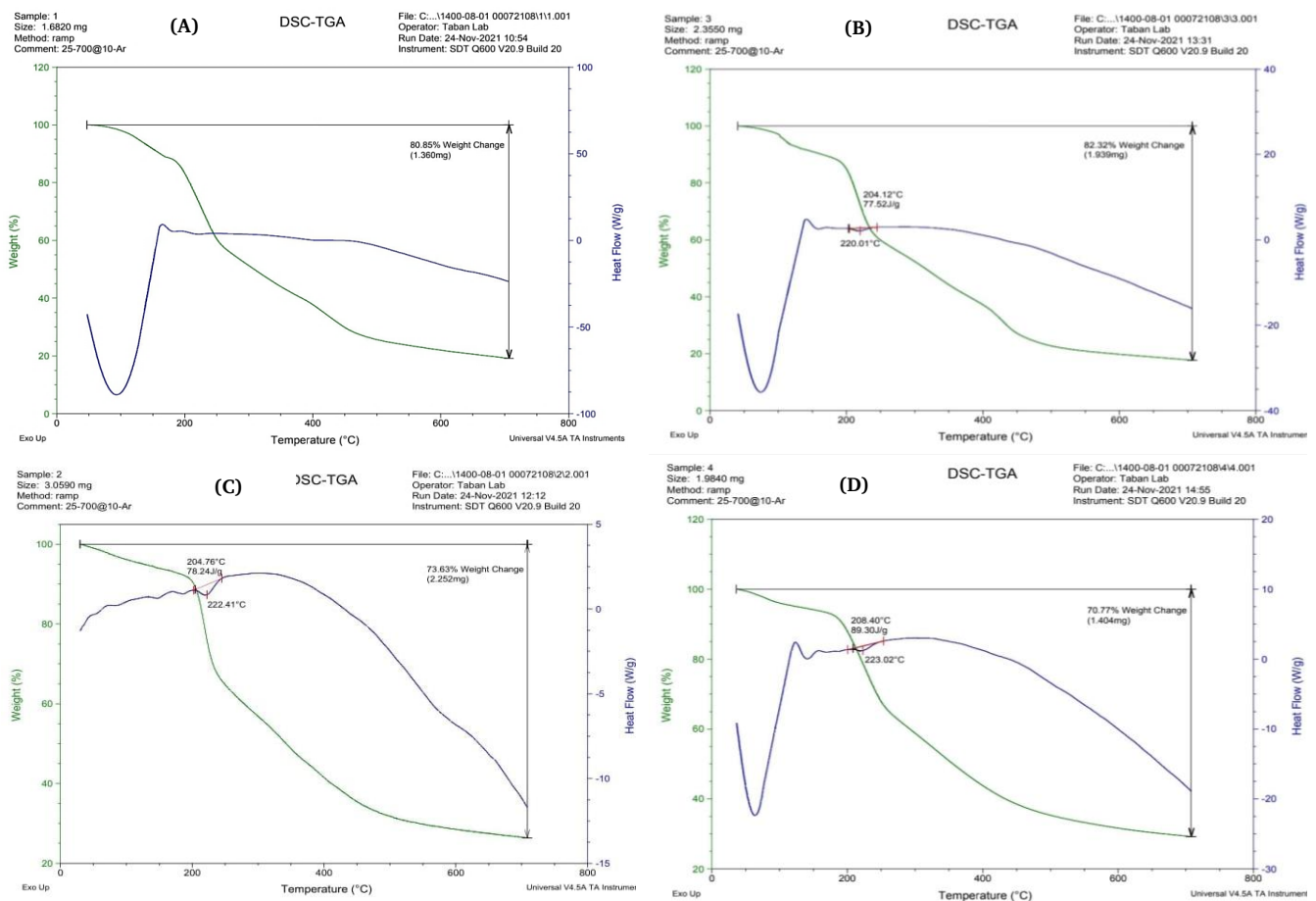
Fig. 3. Thermogravimetric analysis for ice cream Formulas Control (add Guar Gum) IC1 (A), Transglutaminase and Guar Gum (IC2) (B), Gallic acid and Guar Gum (IC3) (C), Transglutaminase and Gallic acid and Guar Gum IC4 (D)
