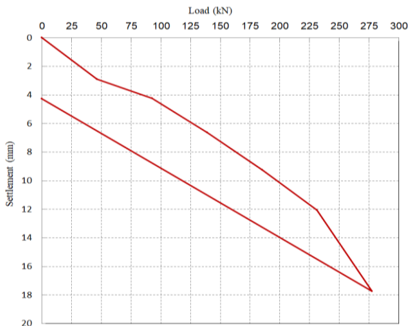
Fig. 7 Relationship between the applied load and the settlement for the tested roof
