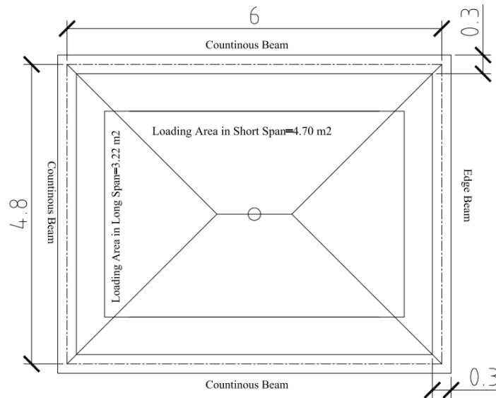
Fig. 3 Block load distribution for half portion in long and short direction of slab orientation
