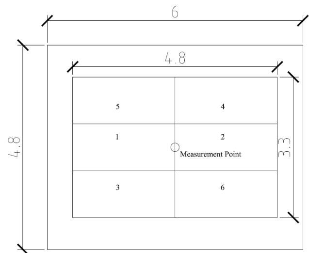
Fig. 1 RC block sequence placement for roof test monotonic load test
