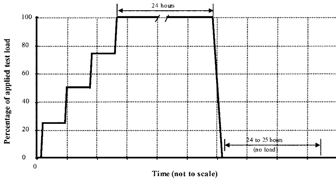
Fig. 2 Loading protocol for the monotonic load test procedure
