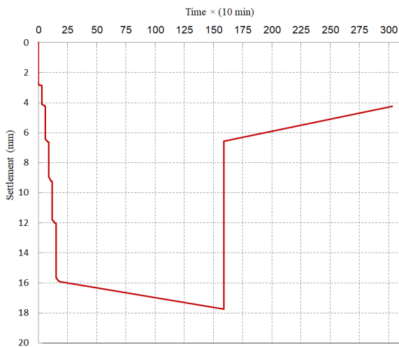
Fig. 6 Relationship between the time and the settlement for the tested roof
