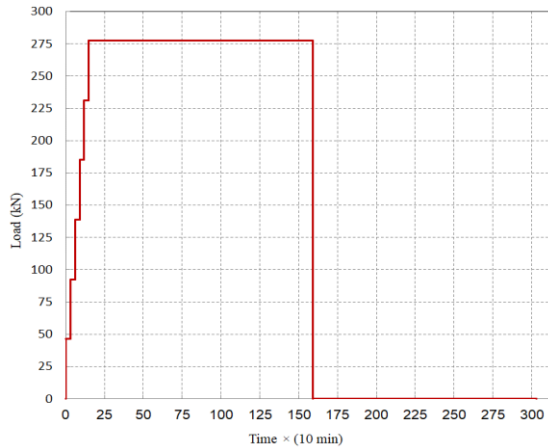
Fig. 5 Relationship between the time and the applied load for the tested roof
