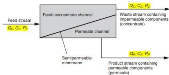
Figure 3. The schematic of separation process through reverse osmosis membrane [4].
