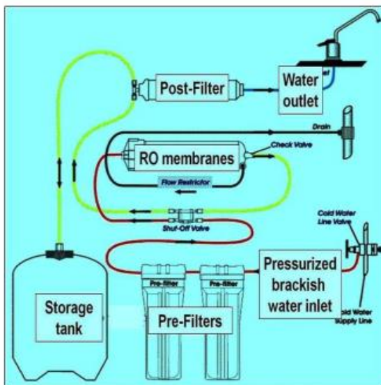
Figure 1. Schematic representation of RO systems [4].
