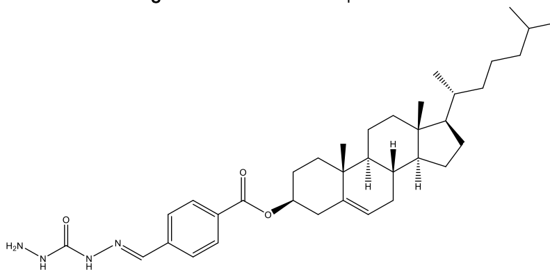
Figure 3. Structure of compound a1
