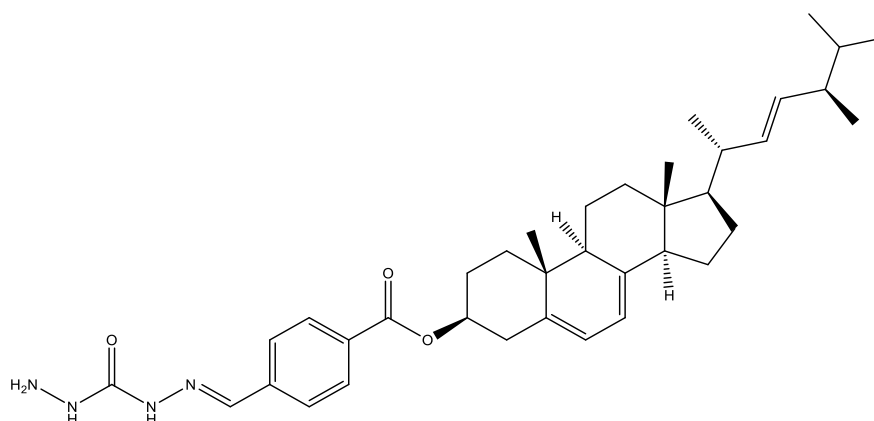
Figure 7. Structure of compound a2
