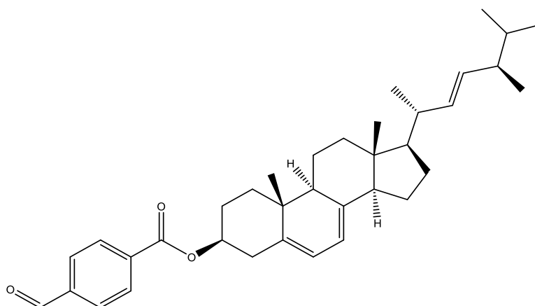
Chemical Formula: \text{C}_{36}\text{H}_{48}\text{O}_3 Molecular Weight: 528.78
