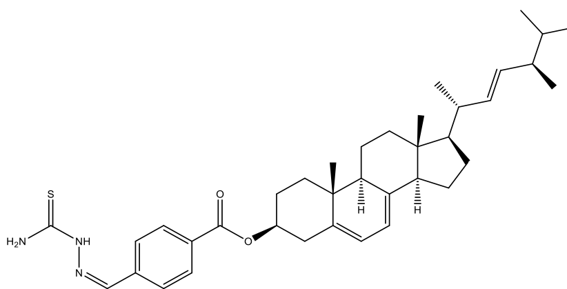
Chemical Formula: \text{C}_{37}\text{H}_{51}\text{N}_3\text{O}_2\text{S} Molecular Weight: 601.89
