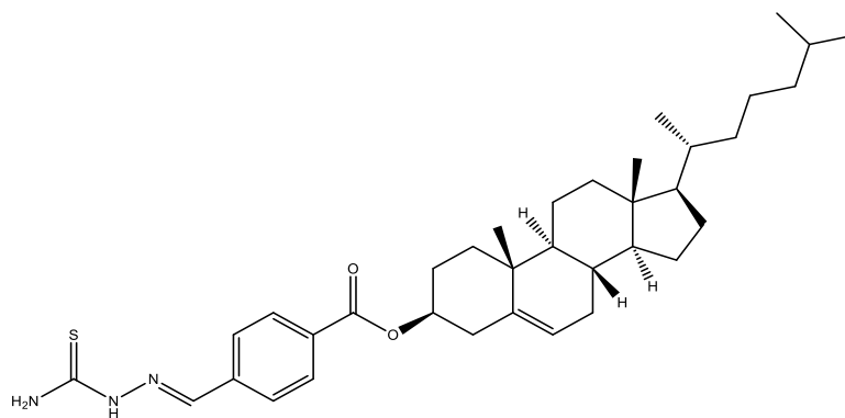
Figure 2. Structure of compound t1
