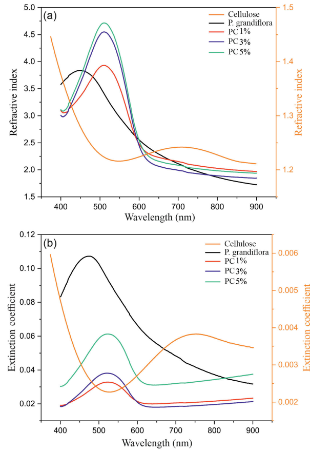
Fig. 9. (a) Refractive index and (b) extinction coefficient vs. wavelength of pure dye, cellulose, and different concentrations of dye-doped cellulose.
