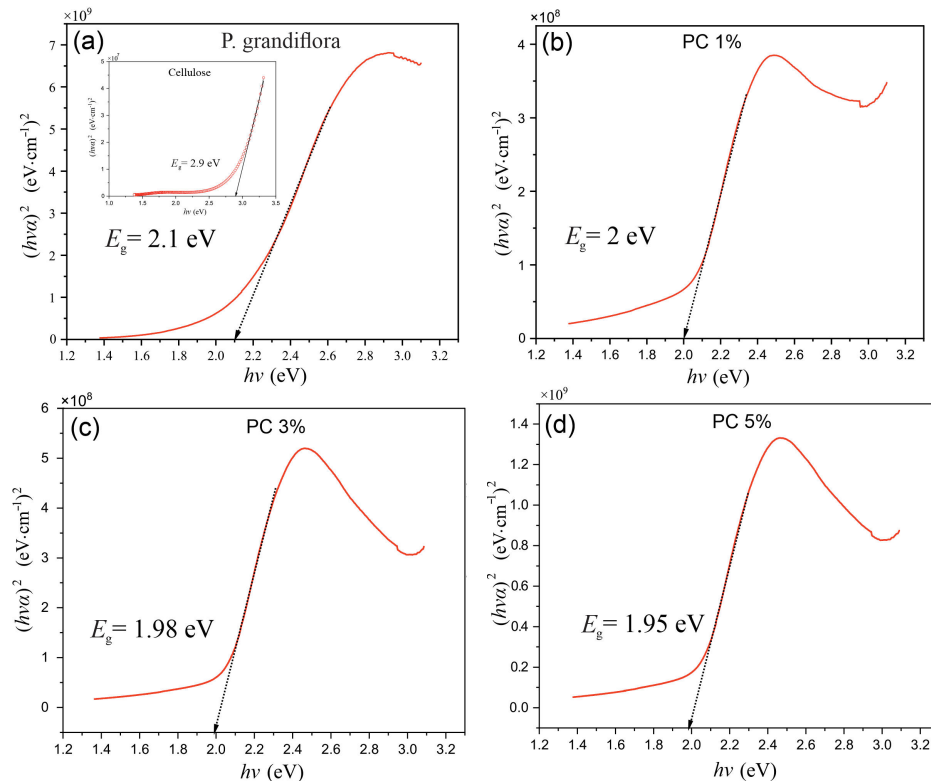
Fig. 7. Energy bandgap of (a) pure dye, (b) PC 1%, (c) PC 3%, and (d) PC 5%. Inset of Fig. 7(a) shows energy bandgap of natural cellulose.
