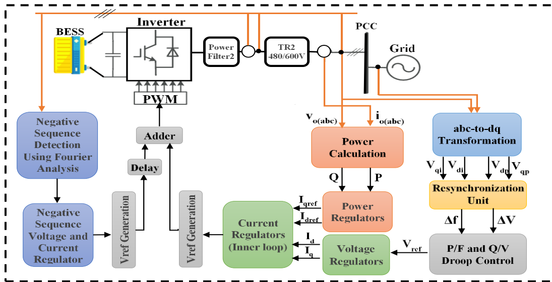
Fig. 11: The proposed control system of BESS inverter
