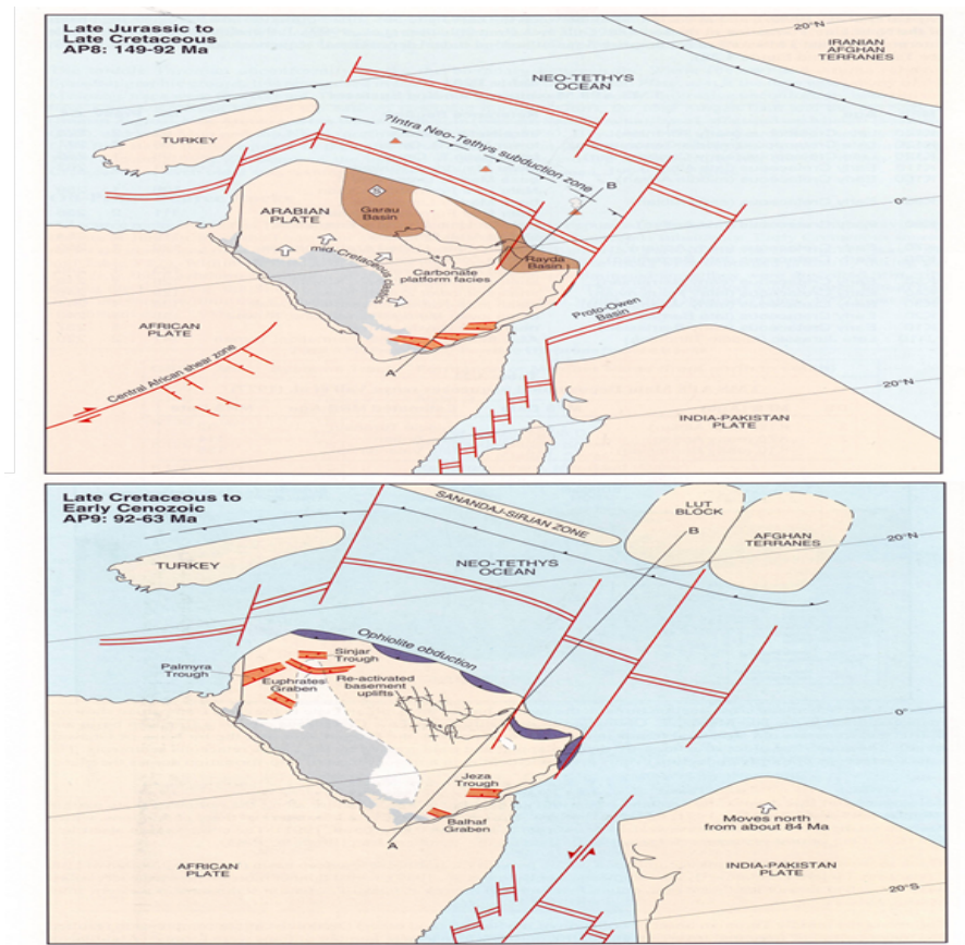
Fig.4. Two tectonic mega sequence phases (AP8, AP9) shown the Arabian plates position during the Cretaceous period Sharland et al.(2000).
