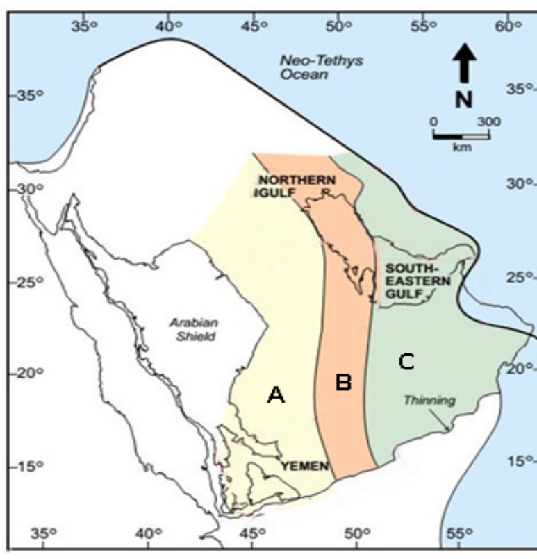
Fig.2. The three longitudinal zones of sedimentations in the Arabian margin during the Early Cretaceous (A) the carbonates zone; (B) the mixed of clastic and carbonates zone, and (C) the clastic zone (Davies et al., 2002).
