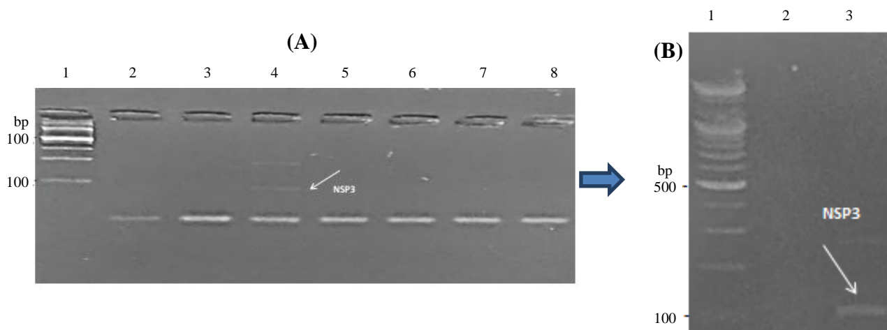
Fig. 1. Agarose gel electrophoresis of PCR-amplified products of rotavirus species-specific primers (NSP3) using: (A) 2% agarose: lane 1, 100 bp DNA size marker; lane 2, no template (negative) control; lanes 3-8 the examined sample. (B): 5% agarose: lane 1, 100 bp DNA size marker; lane 2, no template control; lane 3, an examined sample.
