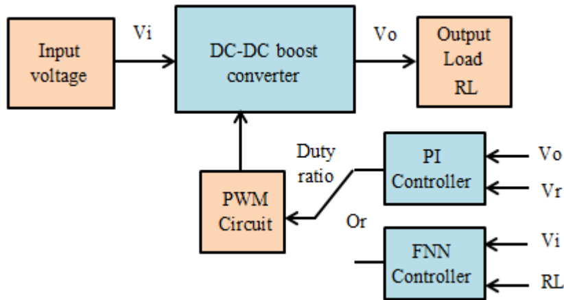
Figure 3. Block diagram of voltage tracking control
