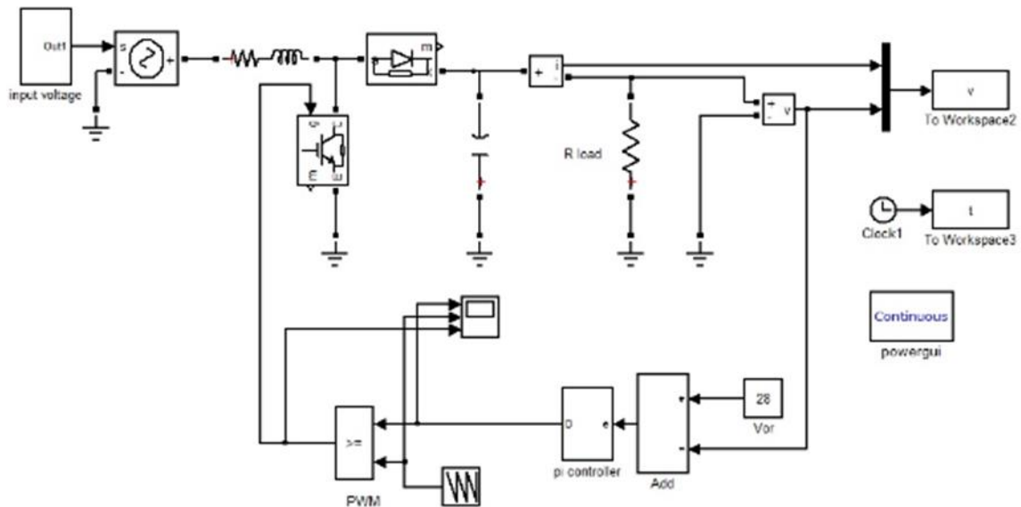
Figure 4. Simulink implementation of PWM Boost Converter based on PI controller
