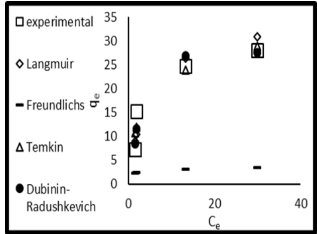
Fig. 12, Comparison between experimental and model isotherms for ibuprofen
