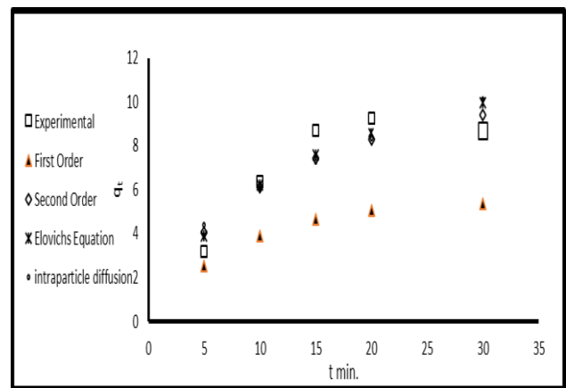
Fig. 8, comparison between experimental and different kinetics models for ibuprofen at temperature 10°C
