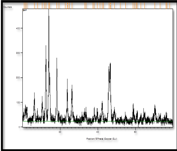
Fig. 15, XRD for Bentonite poly urea formaldehyde composite
