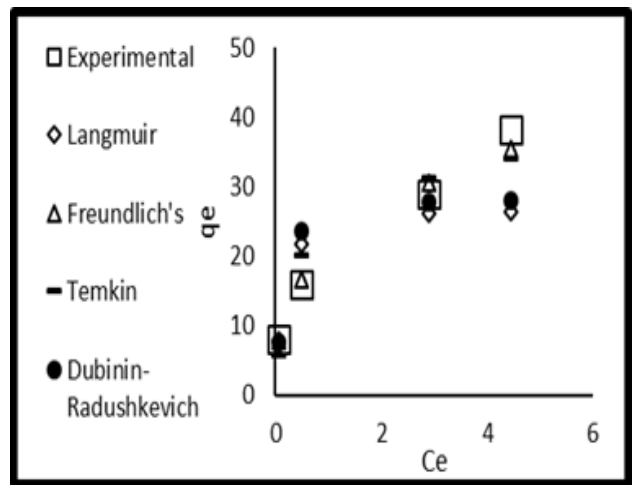
Fig. 13, Comparison between experimental and model isotherms for diclofenac sodium
