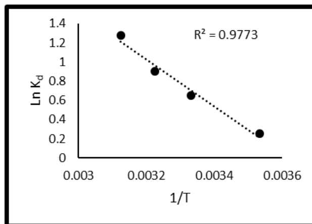
Fig. 7, Determination of thermodynamic parameters ( \Delta G^\circ , \Delta S^\circ & \Delta H^\circ ) for the adsorption, of diclofenac sodium
