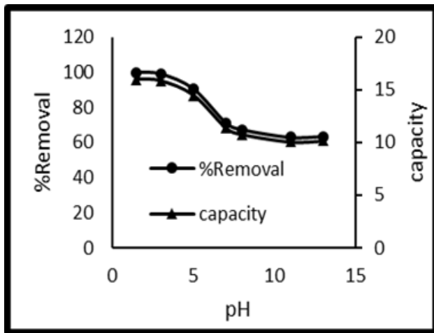
Fig. 11, Effect of pH on both adsorption capacity and removal efficiency of diclofenac sodium, experiment conditions (adsorbent mass =0.05g,r.p.m=180,intial concentration =40µg/ml, temperature =47°C and contact time 15 min).
