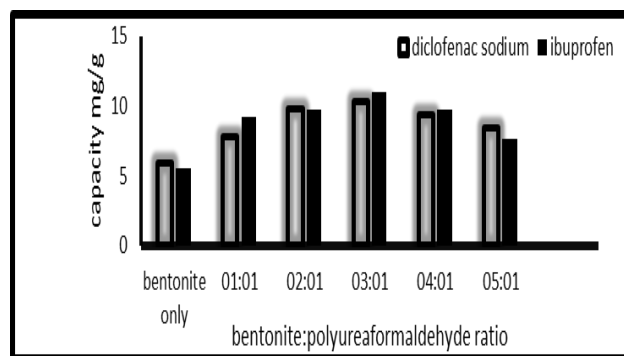
Fig. 3, Effect of composite mass ratios on ibuprofen and diclofenac sodium adsorption, parameters conditions ,pH=7,contact time 3h ,adsorbent mass 0.05g ,sample volume 20 ml, mixing speed 180 r.p.m and initial concentration 40 µg/ml
