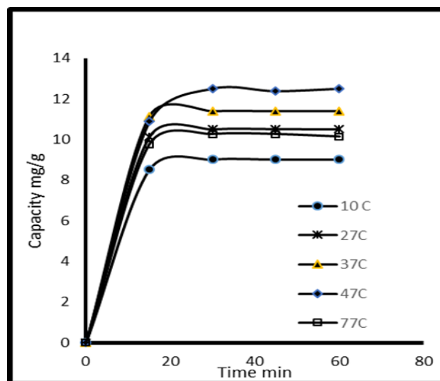
Fig. 5, Interaction between temperature and contact time on adsorption capacity of diclofenac sodium initial concentration of 40 \mu\text{g/ml} ,pH=7and 0.05 g adsorbent weight
