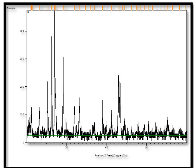
Fig. 14, XRD of Bentonite
