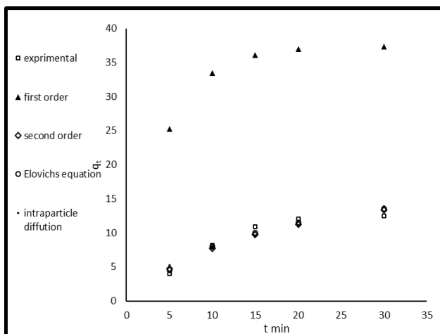
Fig. 9, comparison between experimental and different kinetics models of diclofenac sodium at temperature 47°C
