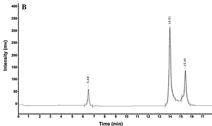
Figure 3 HPLC chromatogram of reuterin compound. (A)standard solution, (B)sample solution.
