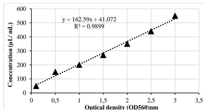
Figure 4 Standard curve of standard acrolein concentrations at optical density (OD) at wavelength 560 nm.
