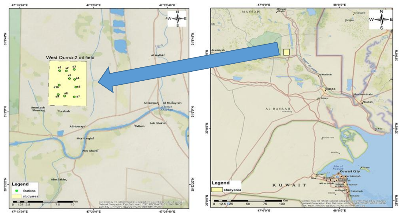
Fig. (1) The study area showing sample locations.
