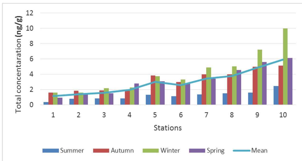
Fig. (2) Seasonal and mean concentration of polycyclic aromatic hydrocarbons at west Qurna- 2 oil field.
