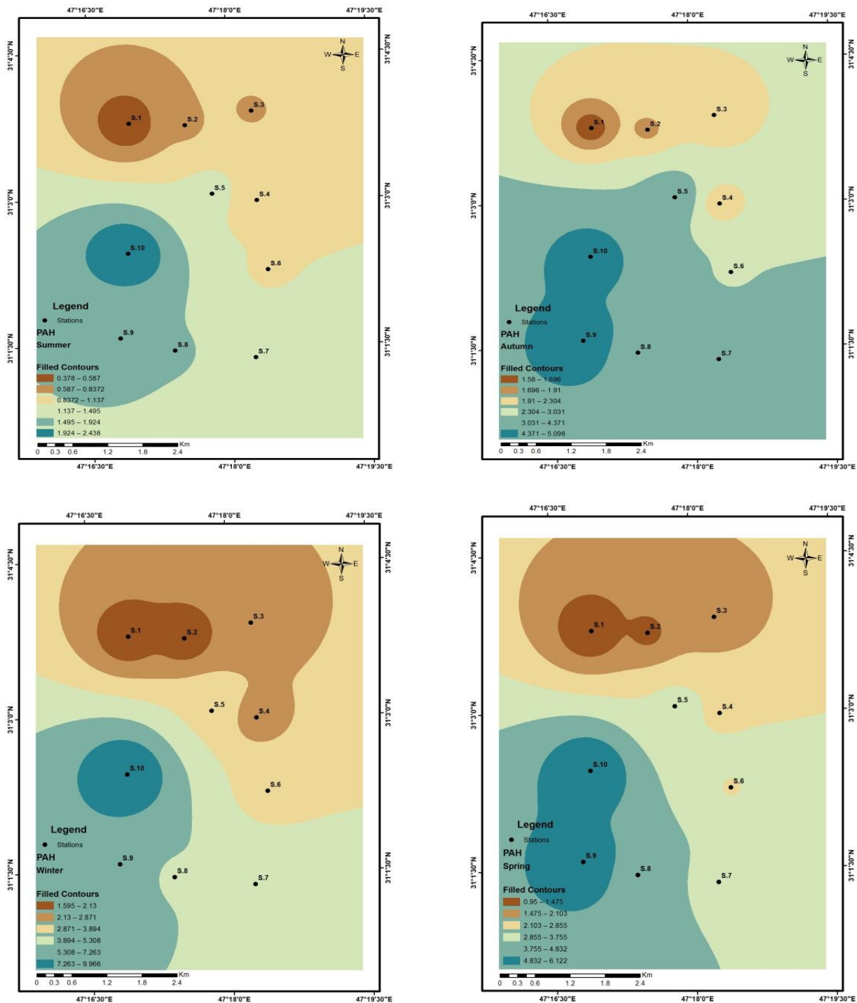
Fig. (3) GIS map showing polycyclic aromatic hydrocarbons distribution in soil at west Qurna- 2 oil field for different seasons.
