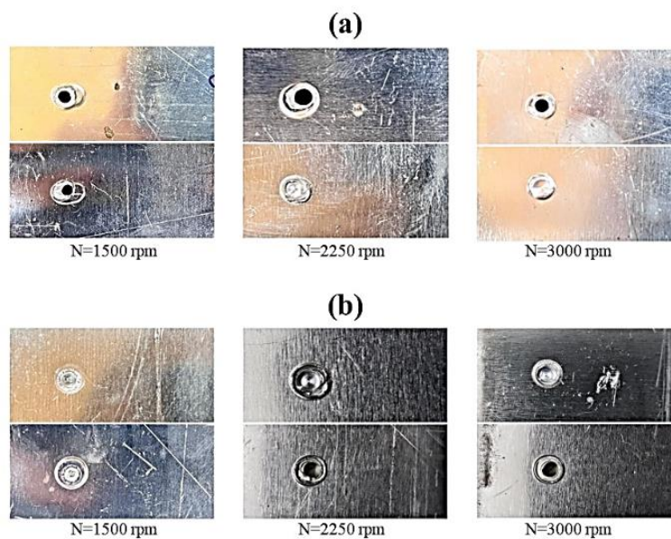
Fig. 6. Mechanical failure at a) pin d=3\text{mm} and b) pin d=4\text{mm}
