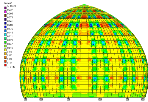
FIGURE 26. Meridional Stresses of RD#5, having in plan theta angle 30° and rings spacing 1.5 m
