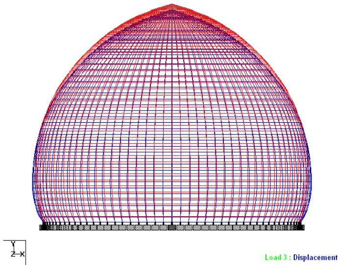
FIGURE 3. Deflection Shape and maximum deflection results of BD#1
