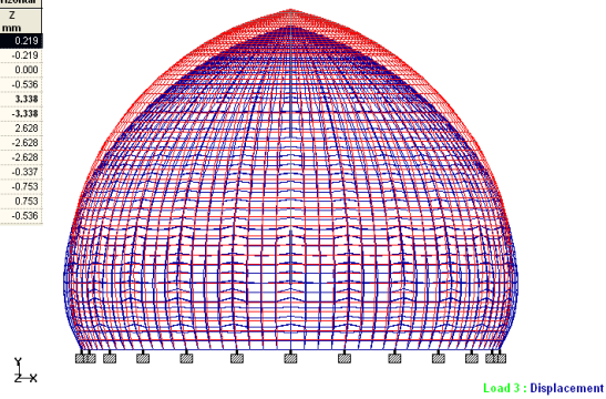
FIGURE 12. Deflection Shape and maximum deflection results of RD#1, having in plan theta angle 15° and rings spacing 1.5 m
