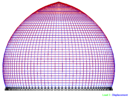
FIGURE 6. Deflection Shape and maximum deflection of BD#2
