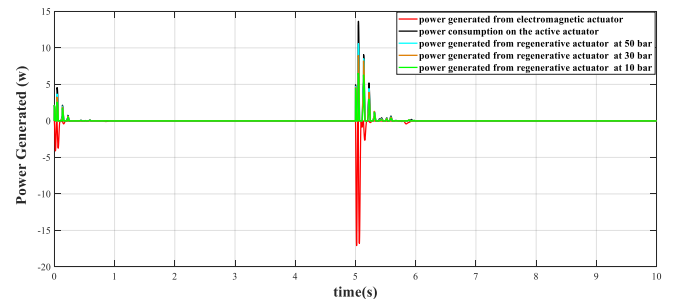
Fig. 15 Comparison of power at the FL suspension.
