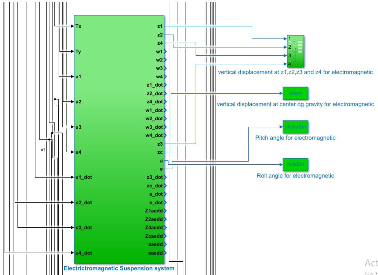
Fig. 3 Full-vehicle active and regenerative suspension systems block diagram.
