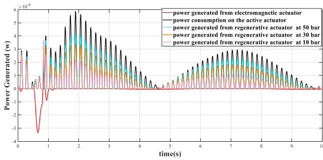
Fig. 13 Comparison of power at the RR suspension.
