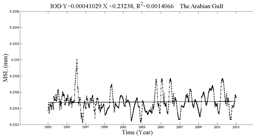
Figure 1. The linear trend of IOD in the Arabian Gulf
