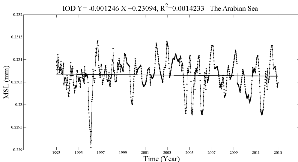
Figure 2. The linear trend of IOD in the Arabian Sea
