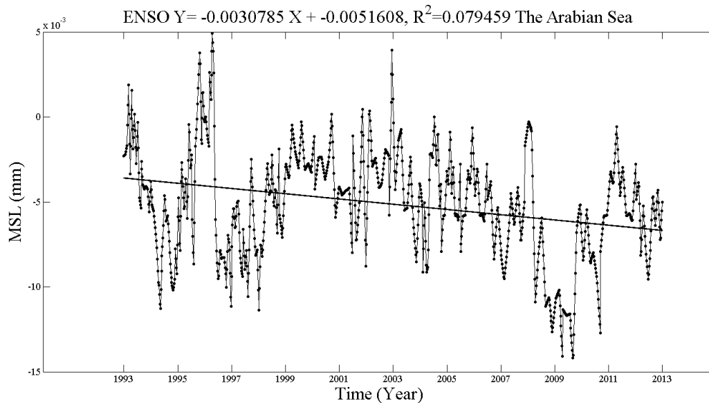
Figure 3. The linear trend of ENSO in the Arabian Sea
