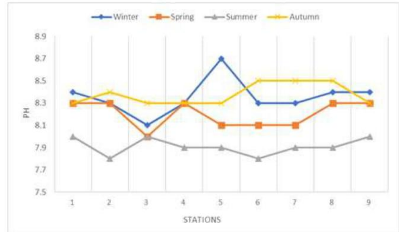
Fig. 5. Hydrogen ion concentration (pH) in SNR
