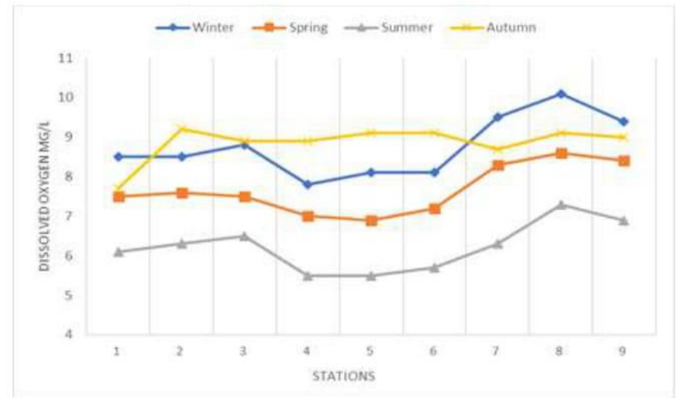
Fig. 9. Dissolved Oxygen (EC) \text{mg L}^{-1} in SNR
