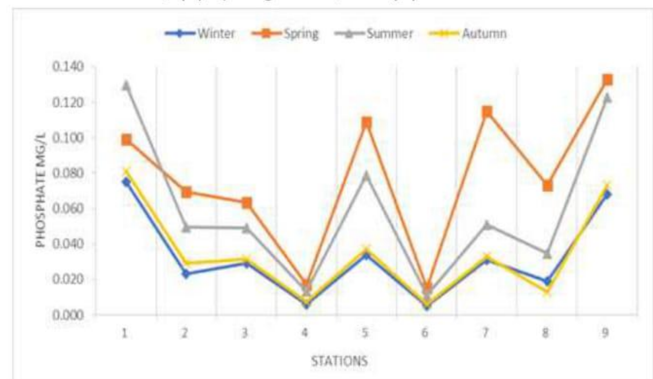
Fig. 13. Phosphate concentration (PO 4 3- ) µg l -1 in SNR
