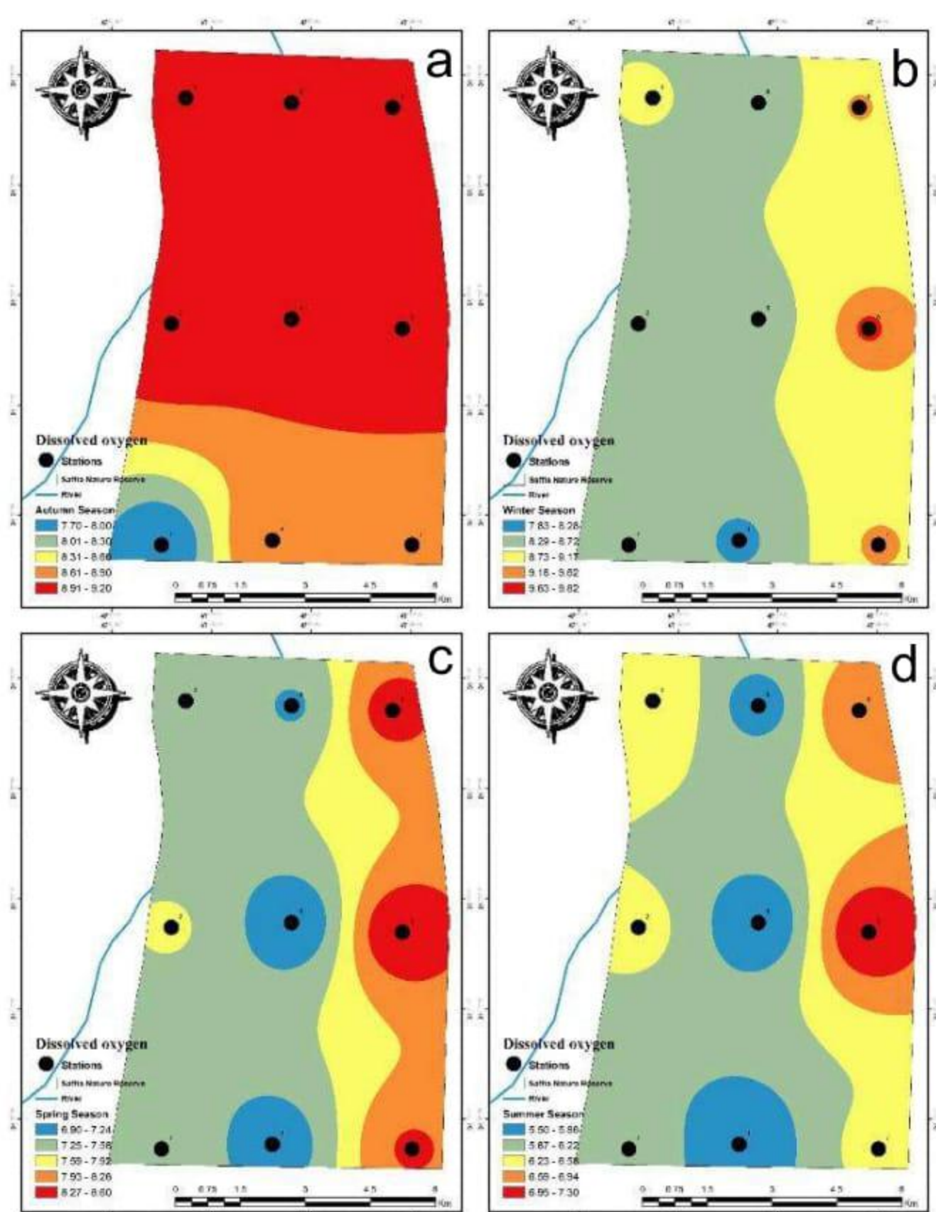
Fig. 10. Spatial distributions of DO \text{mg L}^{-1} values using IDW interpolation: (a) autumn 2019, (b) winter 2020, (c) spring 2020, and (d) summer Season 2020
