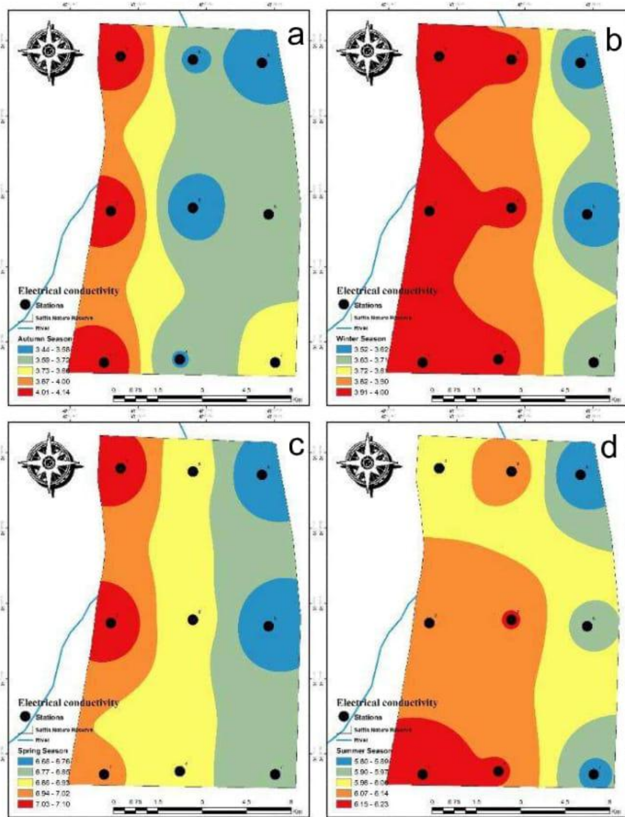
Fig. 8. Spatial distributions of E.C. values using IDW interpolation: (a) autumn 2019, (b) winter 2020, (c) spring 2020, and (d) summer Season 2020
