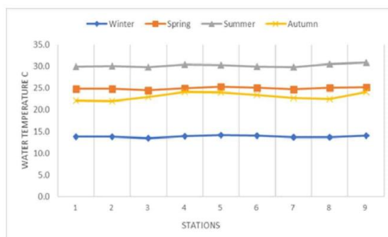
Fig. 3. Water temperature (°C) in SNR
