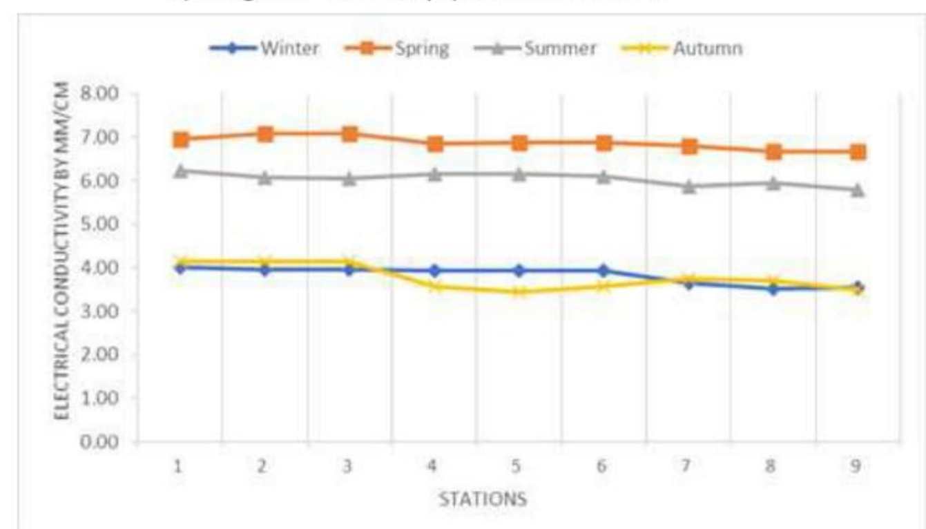
Fig. 7. Electrical Conductivity (EC) \mu\text{m cm}^{-1} in SNR
