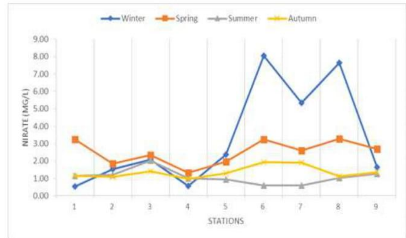
Fig. 11. Nitrate concentration (NO 3 - ) mg L -1 in SNR
