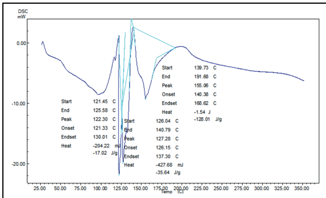
Figure 12. DSC thermogram of uncured phenolic resin (RC).
