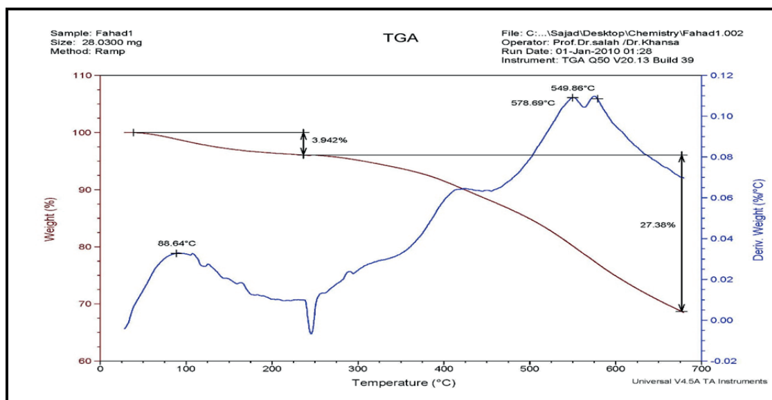
Figure 5. TGA/DTG thermogram of cured (RR) resin.
