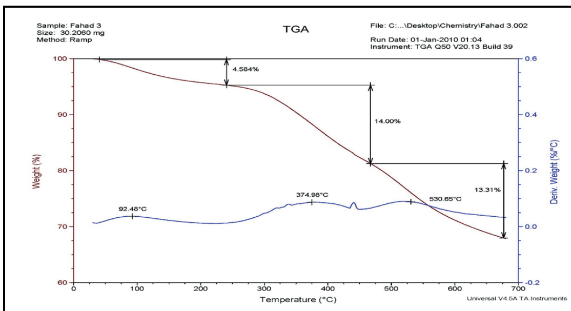
Figure 7. TGA/DTG thermogram of cured (RP) resin
