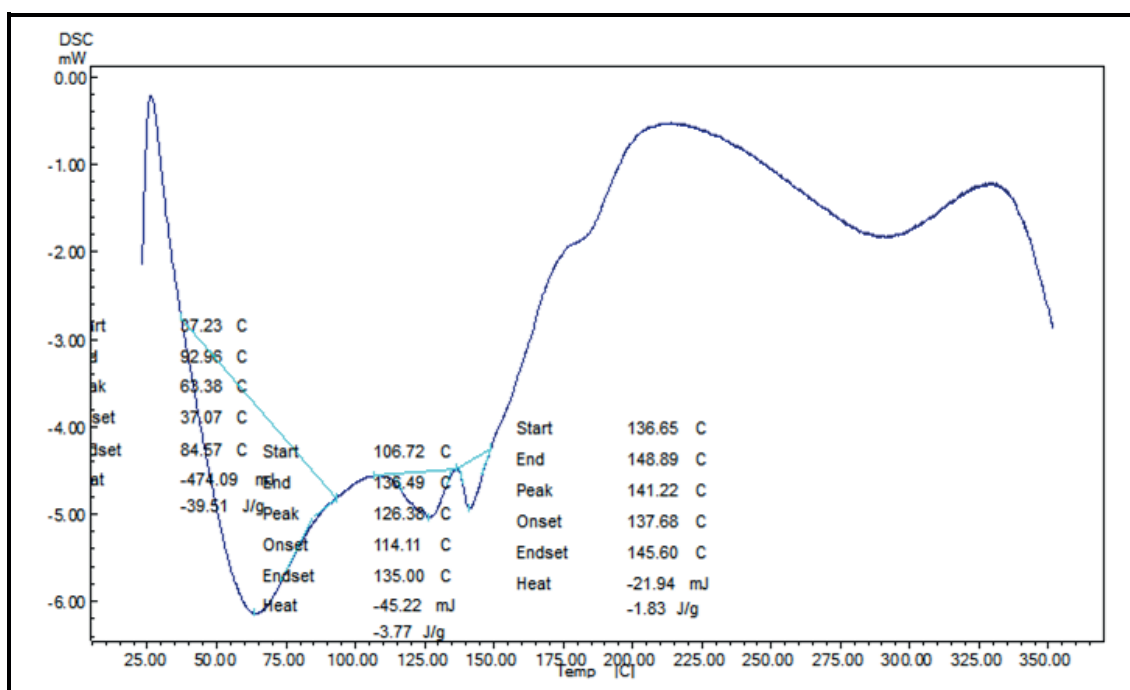
Figure 11. DSC thermogram of uncured phenolic resin (RP).
