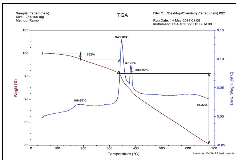
Figure 8. TGA/DTG thermogram of cured (RC) resin.
