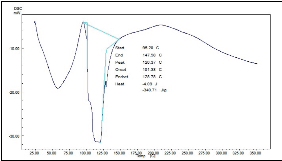
Figure 9. DSC thermogram of uncured phenolic resin (RR)
