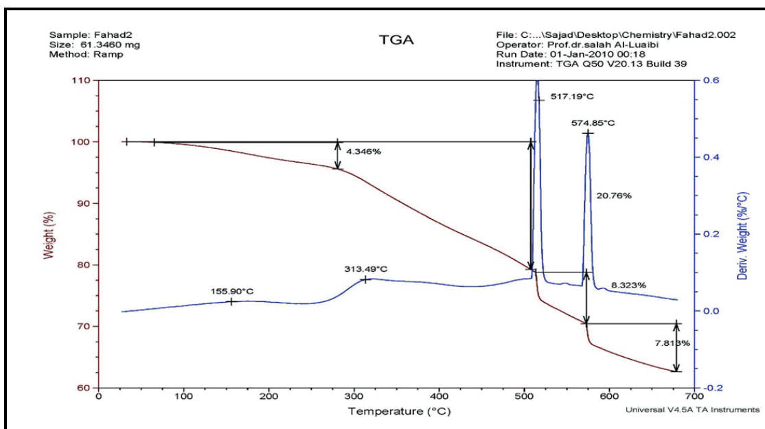
Figure 6. TGA/DTG thermogram of cured (RH) resin.
