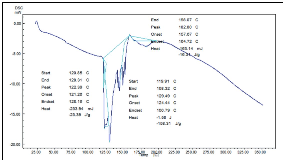
Figure 10. DSC thermogram of uncured phenolic resin (RH).
