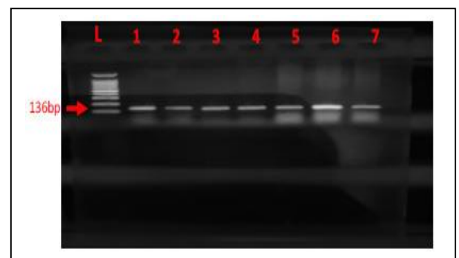
Figure 1. Polymerase chain reaction amplification of Brucella abortus AlkB gene (136bp)
