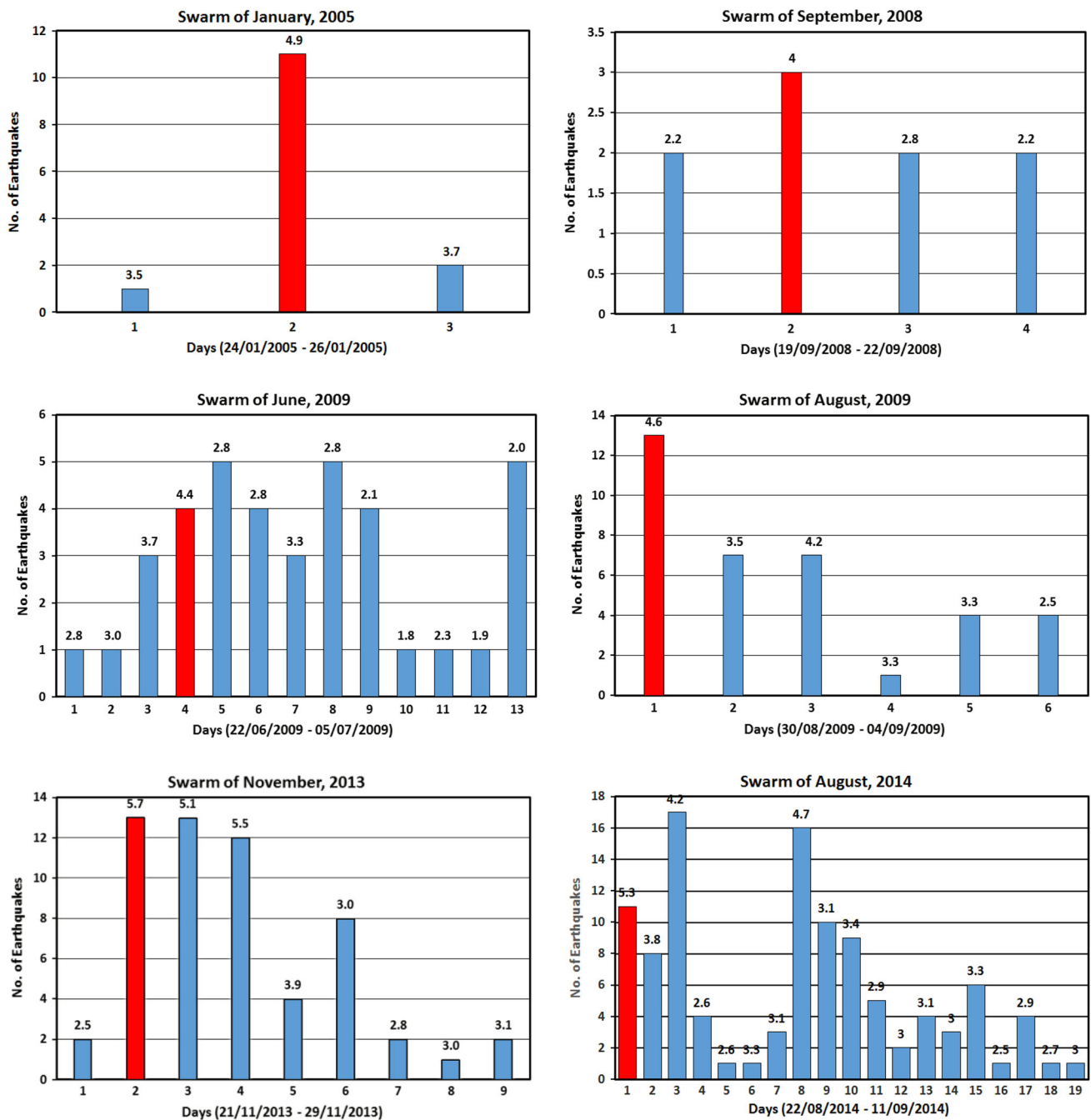
Fig. 4 Graphical descriptions of the six swarms of Diyalah city during 10 years (2004–2014). Red column depicts the day of mainshock. Number above each column represents the highest magnitude during the day
