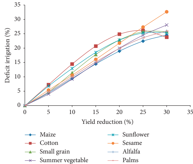
FIGURE 4: Deficit irrigation against yield reduction for eight crops in medium soil.
