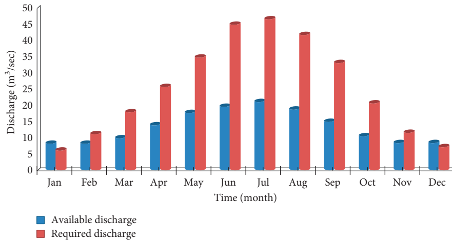
FIGURE 3: Requirements of discharge at the head of the main canal for the period from 2012 to 2018.
