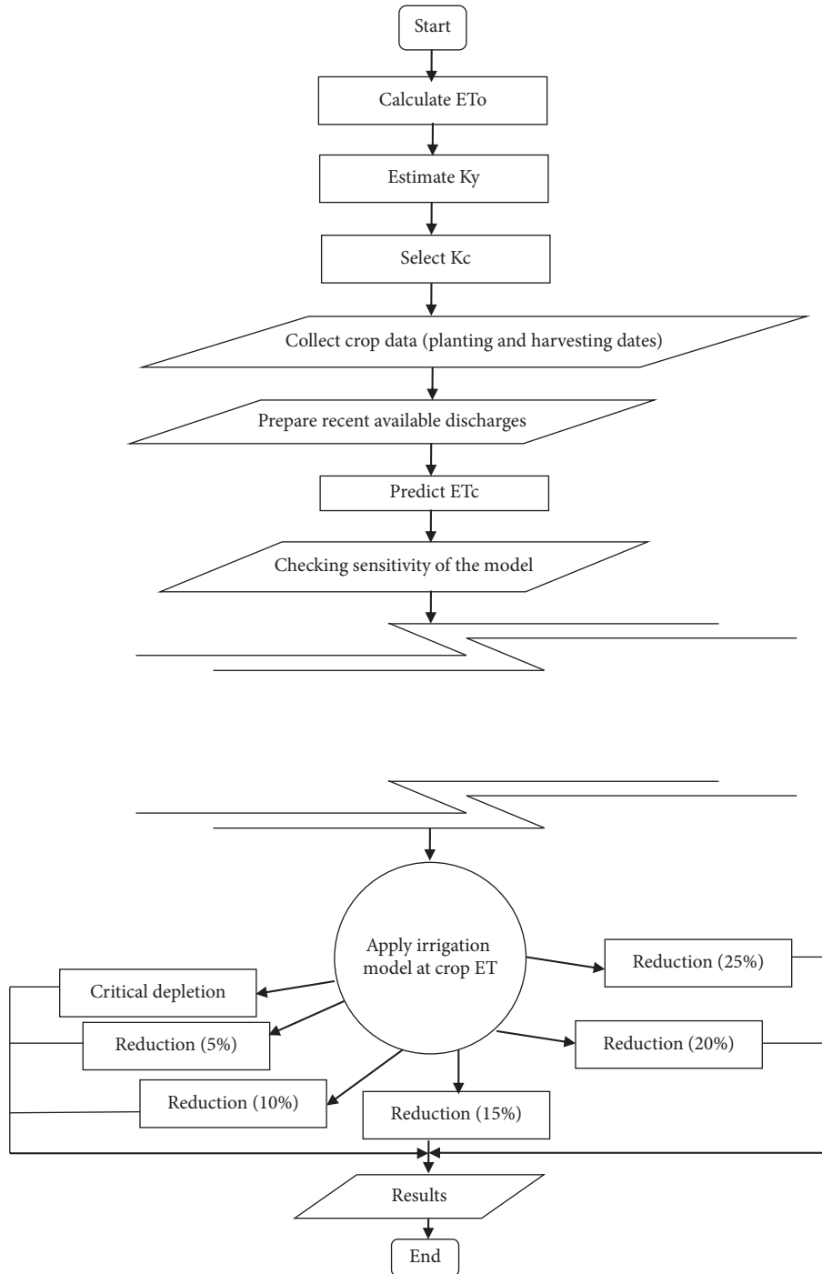
FIGURE 2: Flow chart of methodology for each crop.
