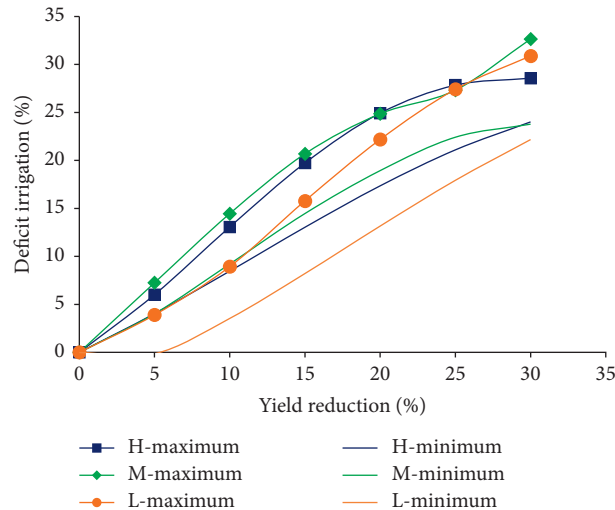
FIGURE 6: Maximum and minimum deficit irrigation against yield reduction for height, medium, and light soil relative to all crops.
