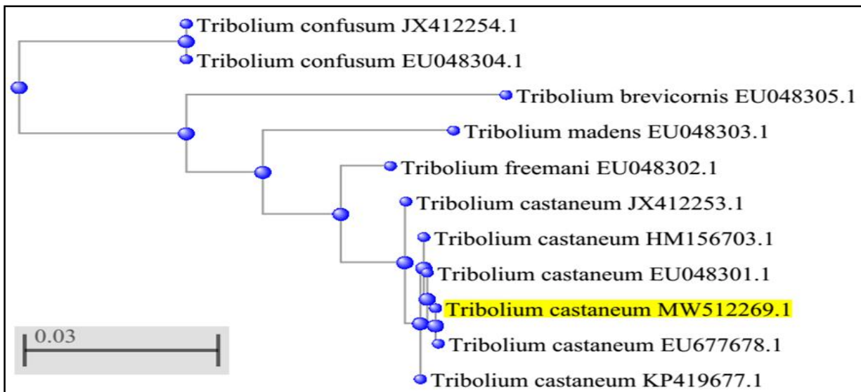
Fig. 1: Genetic relationship tree among the beetle Tribolium castaneum and its comparison with Isolates found in the
