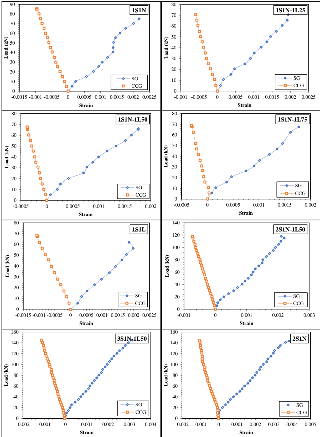
Fig. 10 Load-strain curves.
