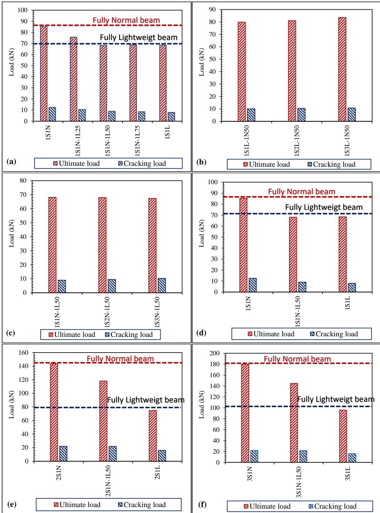
Fig. 9 experimental load of the tested beams.
