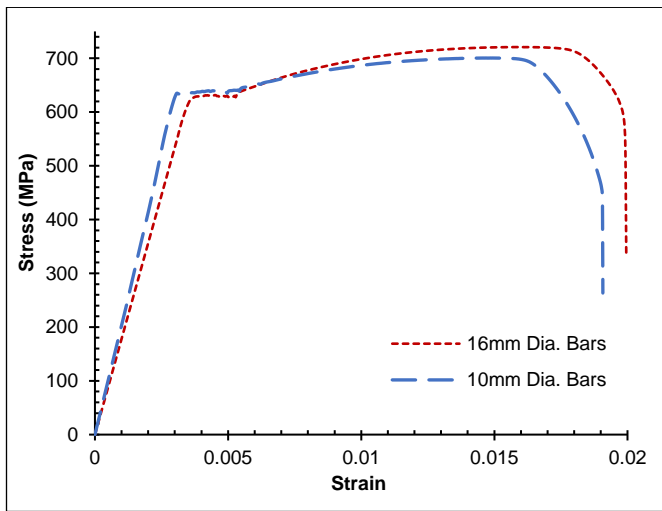
Fig. 1 Stress-strain curves for steel reinforcement bars.
