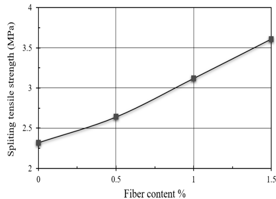
Figure 12. Splitting tensile strength (MPa).
