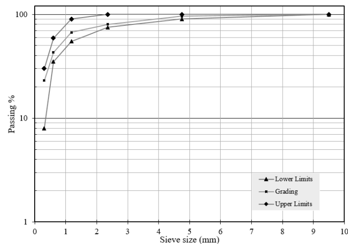
Figure 1. Fine aggregate grading curves.
