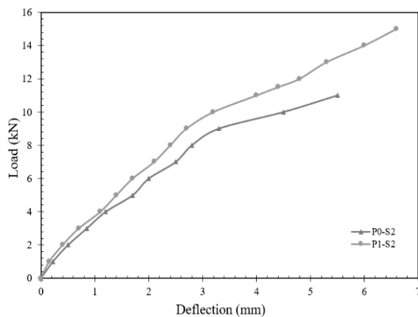
Figure 15. Load–deflection relationship with two polyolefin fiber rates (S2).
