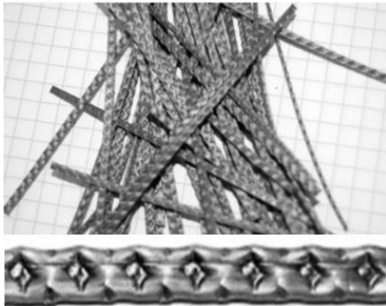
Figure 3. Polyolefin fiber [4].
