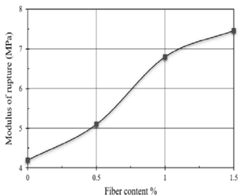
Figure 11. Modulus of rupture (MPa).
