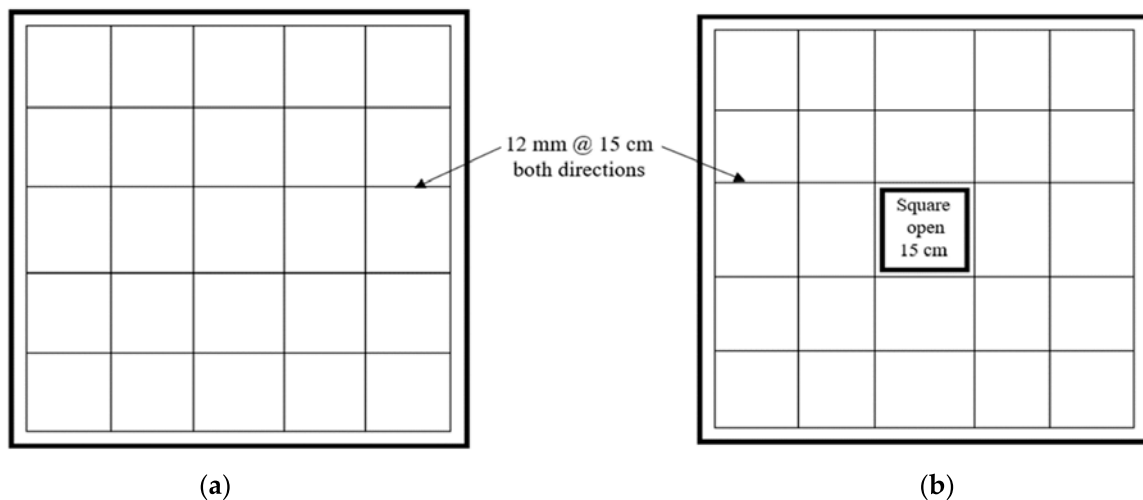
Figure 4. Reinforcement grid for (a): slab set S1, (b) Slab set S2.
