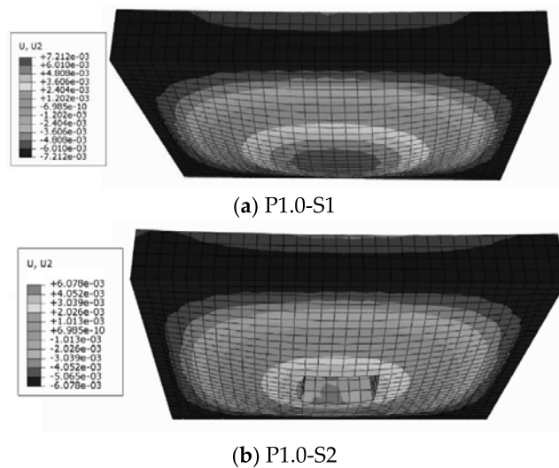
Figure 22. Simulation of deflection for (a) solid slab and (b) Slab with hole.
