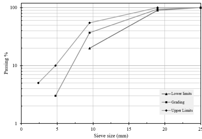
Figure 2. Coarse aggregate grading curves.
