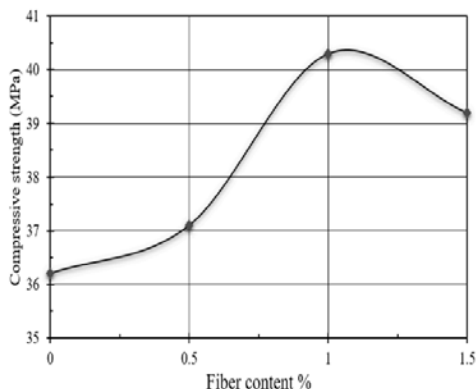
Figure 10. Compressive cube test.
