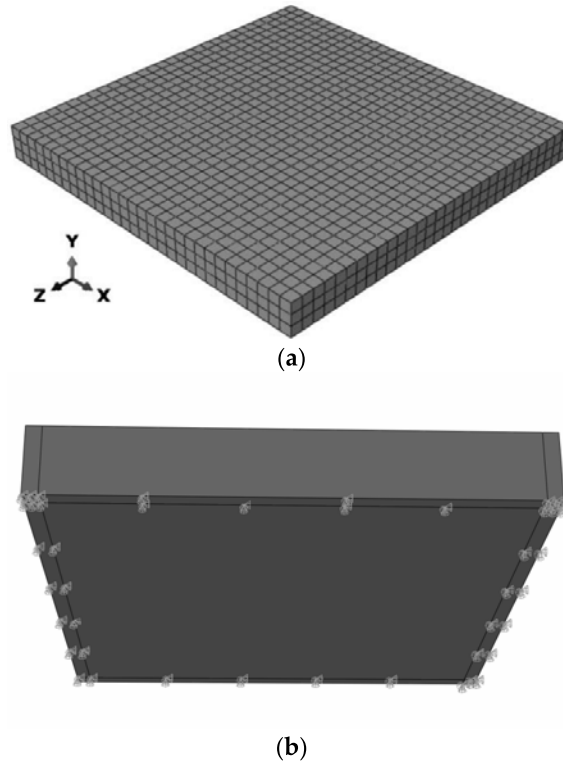
Figure 8. (a) Mesh size. (b) Slab boundary condition.
