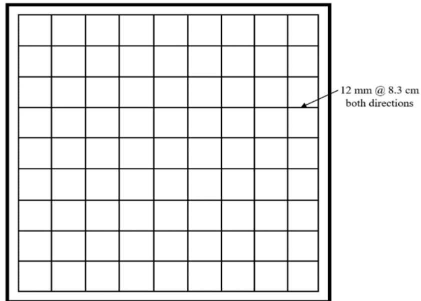
Figure 5. Reinforcement grid for slab set S3.
