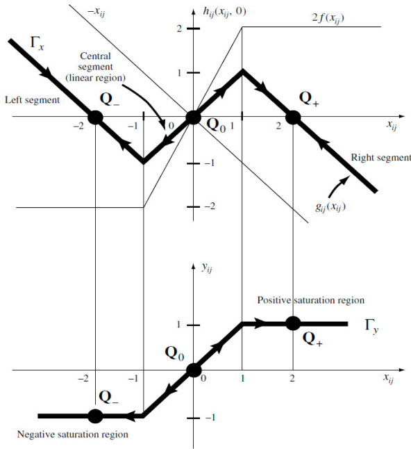
Fig. (5) Dynamics route of both the state x_{ij} and output Y_{ij} with zero offset level ( w_{ij} = 0 ).
