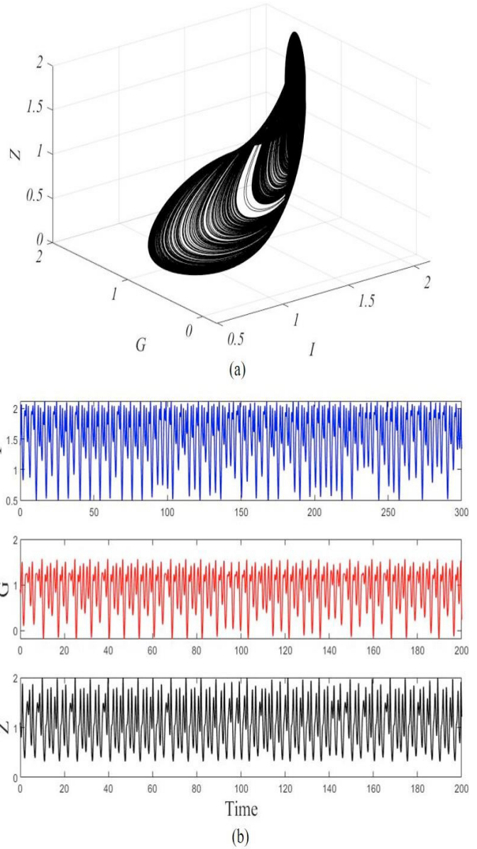
Fig. (2) (a) 3D view of the chaotic response of the insulin-glucose regulatory system and (b) Positive time series of the system.
